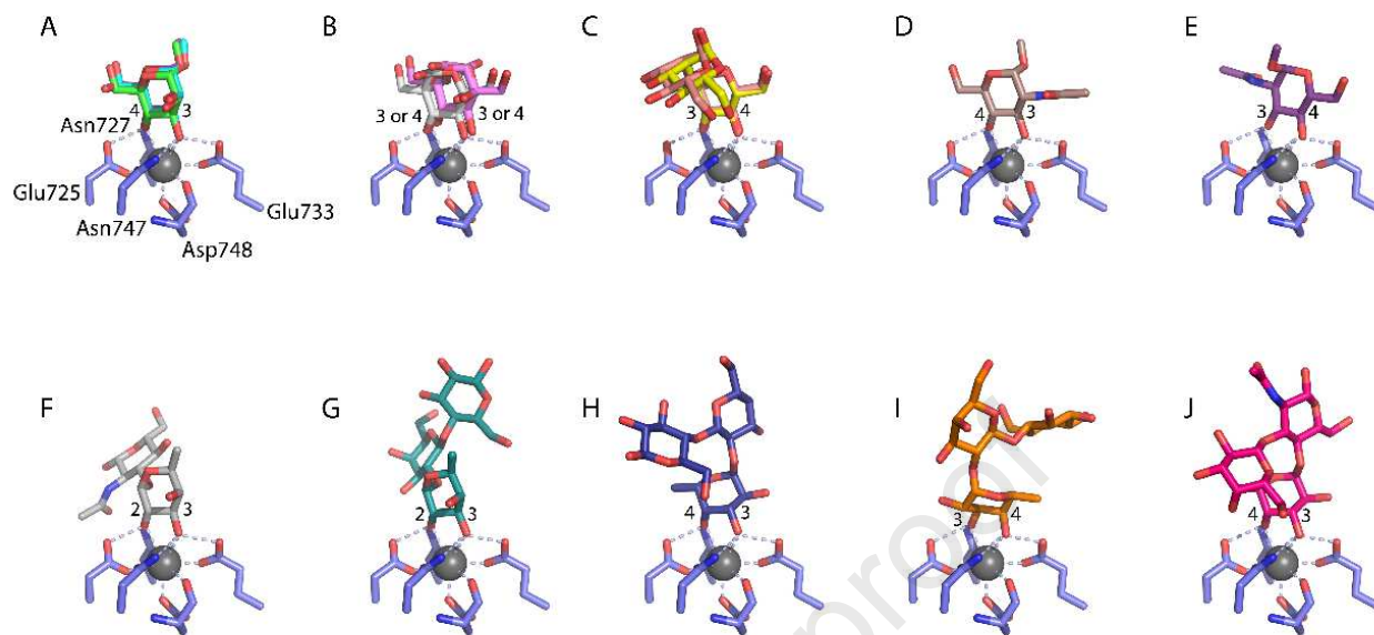
Figure 1. CRD4 primary monosaccharide-binding site interactions demonstrating the promiscuous power of \text{Ca}^{2+} coordination (2). Carbons of the interacting monosaccharide hydroxyl groups are labelled adjacently for all the complexes. \text{Ca}^{2+} is shown as a dark sphere. Amino acids participating in the primary binding site are labelled in A . CRD4 is shown in complex with: A . Methyl- \alpha -D-mannose (three complexes from pdb id 7JUB, 7JUC and 7JUD), B . D-mannose (white, dual occupancy, pdb id 7JUG) and D-mannose- \alpha -1,6-D-mannose (rose, only the non-reducing dual occupancy monosaccharide could be modelled, pdb id 7JUH,), C . D-mannose- \alpha -1,2-D-mannose (two complexes from pdb id 7JUE and 7JUF), D . Methyl- N -acetyl- \alpha -D-glucosamine (pdb id 7L65), E . Methyl- N -acetyl- \alpha -D-glucosamine (pdb id 7L66), F . L-fucose- \alpha -1,3- N -acetyl-D-glucosamine (pdb id 7L67), G . L-fucose- \alpha -1-2-D-galactose- \beta -1-4-D-glucose (pdb id 7L63), H . L-fucose- \alpha -1-2-D-galactose- \beta -1-4-D-glucose (pdb id 7L62), I . L-fucose- \alpha 1-2-D-galactose- \beta -1-4-D-glucose (pdb id 7L61) and J . the Lewis-A trisaccharide (pdb id 7L64).
