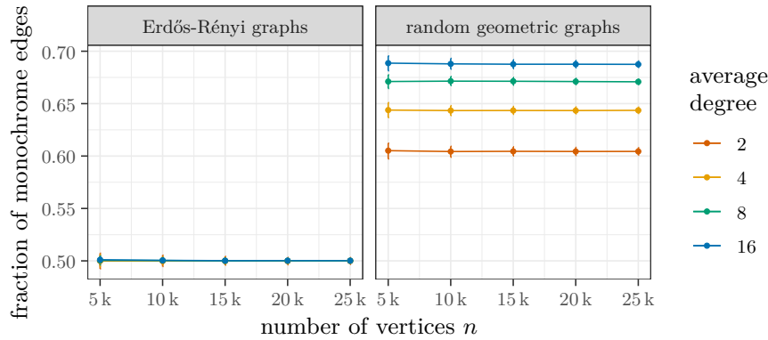
Figure 1 The fraction of monochrome edges after the Flip Schelling Process (FSP) in Erdős-Rényi graphs and random geometric graphs for different graph sizes (number of vertices n ) and different expected average degrees. Each data point shows the average over 1000 generated graphs with one simulation of the FSP per graph. The error bars show the interquartile range, i.e., 50 % of the measurements lie between the top and bottom end of the error bar.
