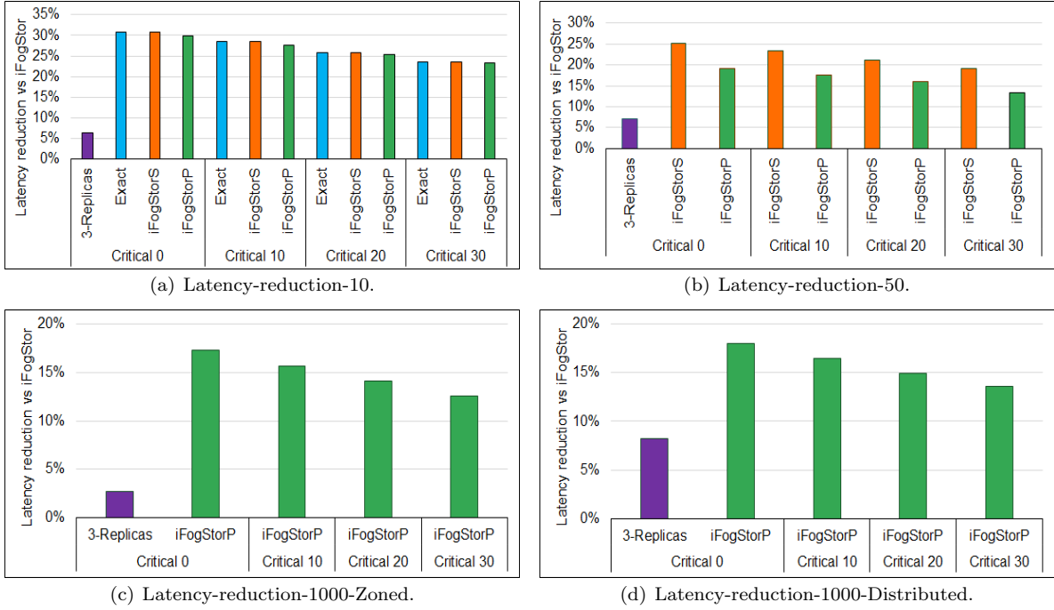
Fig. 11: Latency results.
