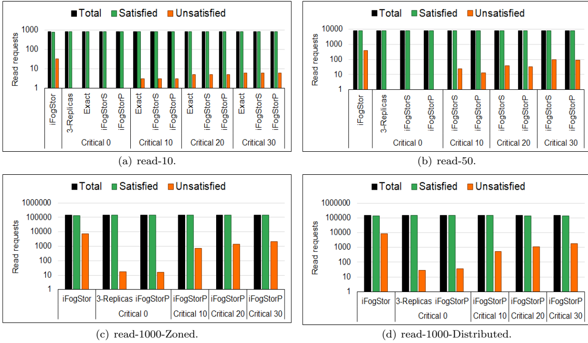
Fig. 14: Read requests results.
