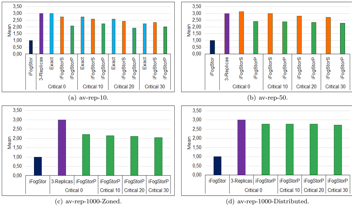
Fig. 13: Replicas number results.
