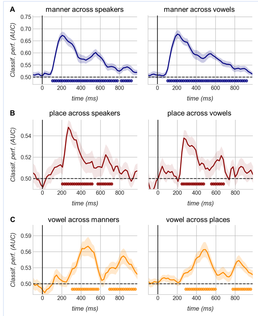
Figure 3: Cross-condition decoding.
