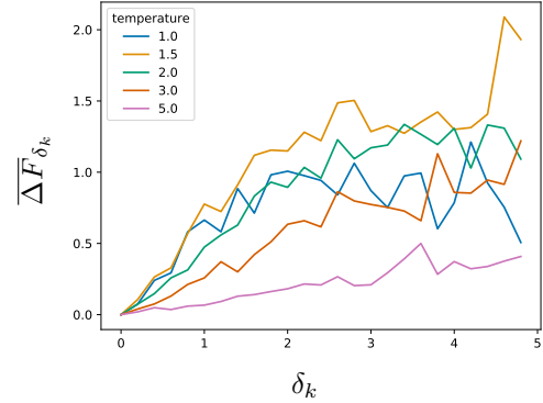
Figure 3. Increment consistency \Delta \bar{F}_{\delta_k} (see Sec.4.4.2)
