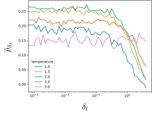
Figure 2. Out-of-distribution average attribute correlation \bar{\rho}_{\delta_l} (see Sec. 4.4.2)
