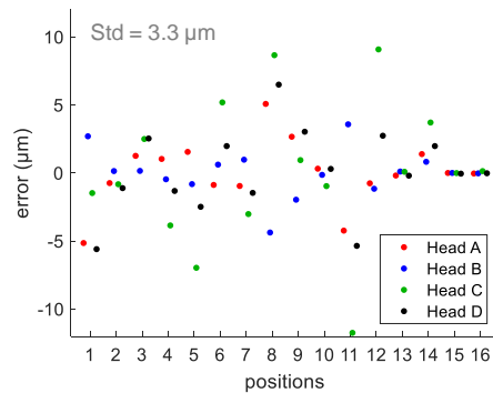
Fig. 21. Experimental results of the multilateration with self-calibration.
