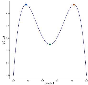
FIG 10. Curve of the variance function in Equation (4) for a Uniform white noise model for m = 1024 , the extrema are reached at p_t \in \{0.172, 0.5, 0.82\} .
