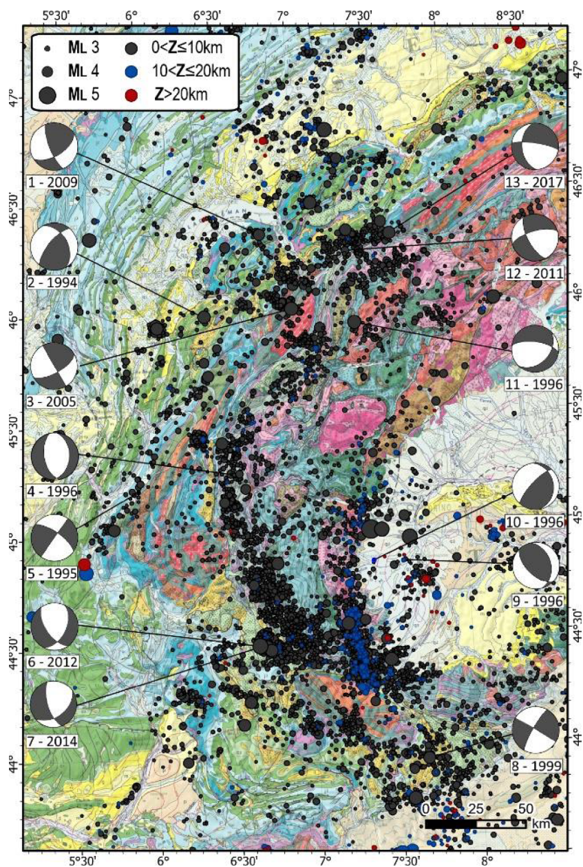
Figure 11. Seismicity overlaid on the geological map of the western Alpine belt, from the CEA_1996–2019 catalog ( M_L \geq 2 ) and Chantraine et al. [2003]. Focal mechanisms: 1. Morzine earthquake [2009/10/21, M_L 3.5; Deichmann et al. , 2012]; 2. Grand Bornand [1994/12/14, M_L 5.1; Fréchet et al. , 1996]; 3. Vallorcine [2005/09/08, M_L 4.9; Fréchet et al. , 2011]; 4. [1996/11/05, M_L 2.5; Béthoux et al. , 2007]; 5. [1995/09/08, M_L 2.5; Thouvenot et al. , 2003]; 6. Barcelonnette [2012/02/26, M_L 4.8; Delouis-Géoazur]; 7. Barcelonnette [2014/04/07, M_L 4.8; Delouis-Géoazur]; 8. Blausasc [1999/11/01, M_L 3.4; Courboux et al. , 2007]; 9. [1996/11/22, M_L 2.3, Béthoux et al. , 2007]; 10. [1996/11/05, M_L 2.4, Béthoux et al. , 2007]; 11. Valpelline [1996/31/03, M_L 4.6; Baer et al. , 1999]; 12. [2011/01/08, M_L 3.5; Deichmann et al. , 2012]; 13. [2017/06/02, M_L 3.3; Diehl et al. , 2021].
