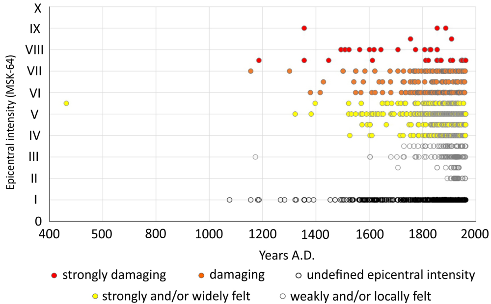
Figure 6. Temporal plot of the historical seismicity recorded in SE France, including the 2055 events of the SISFRANCE database, from year 463 to year 1962. Undefined epicentral intensities are arbitrarily plotted along the I_0 = I axis as presented in Jomard et al. [2021].
