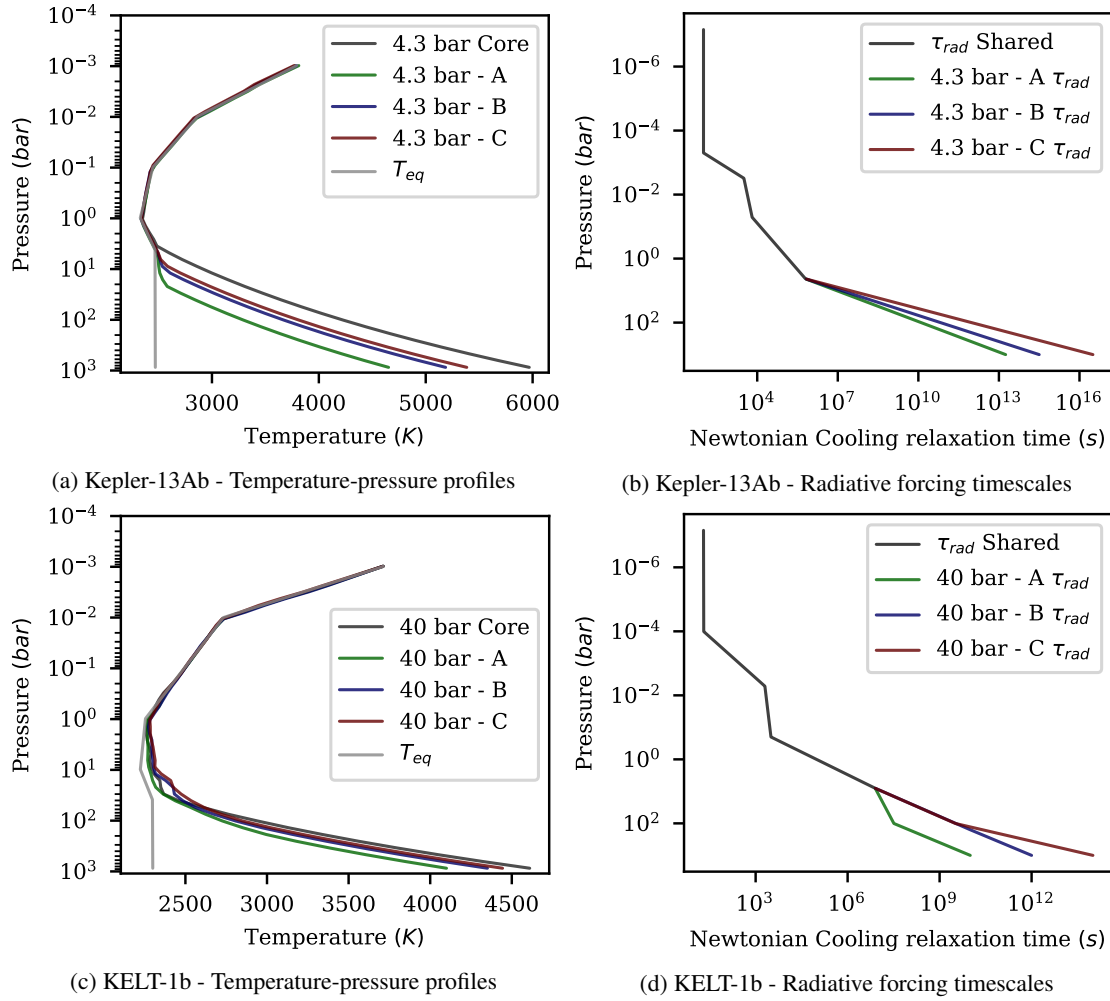
Fig. 8. Snapshots of the T-P profile ( left ) for a series of test models investigating the effect of deep radiative forcing, via deep isothermal Newtonian cooling, on already evolved (dark grey) models of both Kepler-13Ab ( top ) and KELT-1b ( bottom ) with a deeper horizontal convergence pressure. For each brown dwarf, we explored models with increasingly weak deep forcing, as shown by the matching profile on the right, where the full Newtonian cooling timescale profile is found by combining the dark grey profile at lower pressures and the matching coloured profile at higher pressures.
