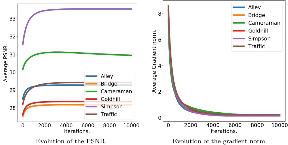
Fig. 8 Convergence diagnosis for Plug & Play deblurring with \sigma^2 = (1/255)^2 , \varepsilon = (5/255)^2 , \alpha = 0.3 and \text{TV} - \text{L}_2 initialization. Left: Evolution of the average PSNR computed for K = 10 independent noise realizations for each of the 6 images. As expected the convergence is slower for the deblurring problem. 4000 iterations seem to be required to enter the stationary phase for all images except Cameraman , that needs on average 1.5e4 iterations. Right: Evolution of the average gradient norm of the log-posterior computed over the 10 experiments for each image. For all images, the gradient norm stabilizes around 0.2.
