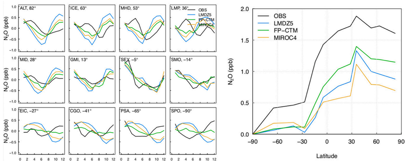
Fig. 16. (Left) Seasonal cycle of N 2 O measured at the surface of 12 stations in 2011 (black) and calculated by LMDz (blue), FLEXPART (green) and MIROC-4 (orange) from the northern to the southern high latitudes. (Right) Observed and calculated annual mean meridional gradient in surface N 2 O with respect to the South Pole station. (For interpretation of the references to colour in this figure legend, the reader is referred to the web version of this article.)
