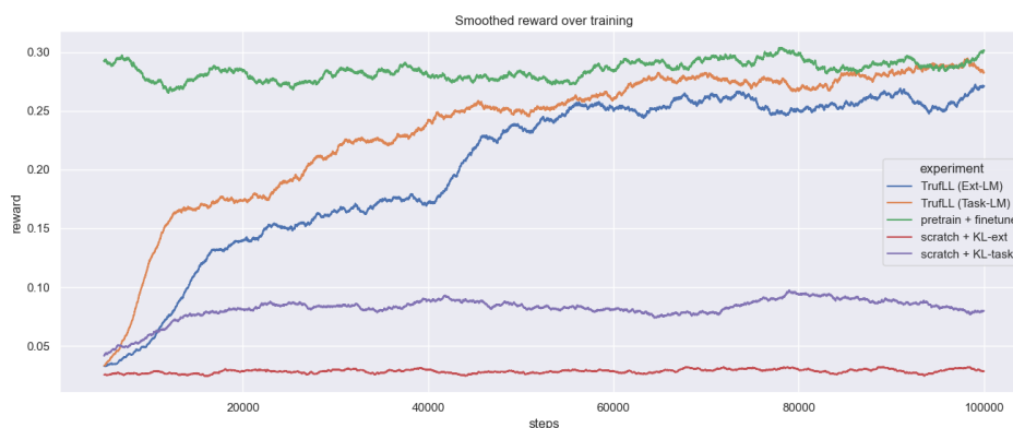
Figure 4: VQA2 : Training curves. Reward is a rolling average over 5000 timesteps.
