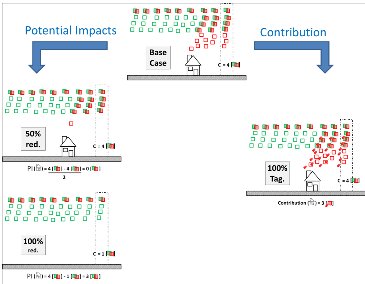
Figure 8: Example of dynamic and non-dynamic SA components. One source (residential) emits gas-phase precursors (red empty squares - \text{NO}_x ) which combine with \text{NH}_3 (green empty squares) to form particulate matter (mixed shaded squares) measured at a given location (dashed rectangle). On the left side, the strength of the residential source is reduced by 50% and 100% to obtain potential impacts (PI) on PM concentrations. On the right side, the residential source emissions are tagged to obtain its contribution. In this figure, the shaded green square represents the modelled ammonium, the shaded red square the modelled nitrate and the mixed green-red shaded pair the modelled ammonium nitrate.
