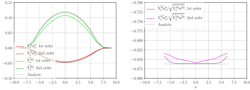
FIGURE 10. Self-similar test case: numerical and analytical solutions on a mesh having a geometric progression, at t = 10 , with N = 50 . The results from the first-order (solid curves), second-order (dashed curves) schemes and the analytical solution (dotted curves) are given for the mass fraction (blue), mass fraction fluxes (red), and mass fraction covariances (green), and the slow variable (purple).
