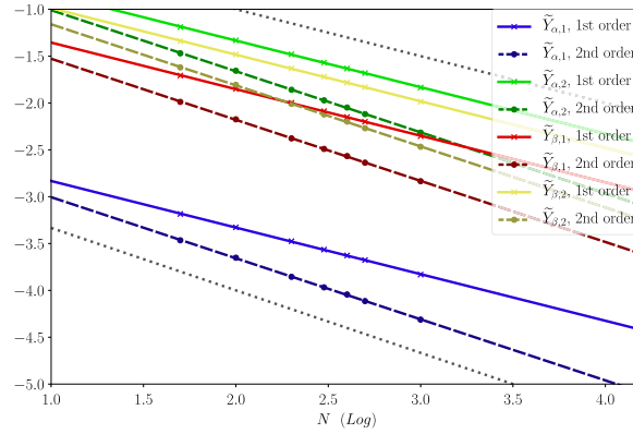
FIGURE 6. Riemann problem: convergence study for the material constituents. Logarithm of the L_1 -error against \log N . The dotted lines correspond to a 1/2 and 2/3 slope, close to the observed convergence rates 0.497 and 0.65 , for the first-order and the second-order schemes, respectively. The symbols correspond to the different mesh refinements. The associated best-fit lines are also shown.
