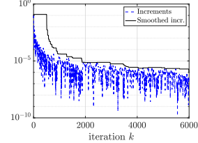
Fig. 1: Stopping criterion. (Normalized) Objective function increments and non linearly smoothed increments as functions of the number of iterations in Algorithm 1 (computed from new infections in France).
