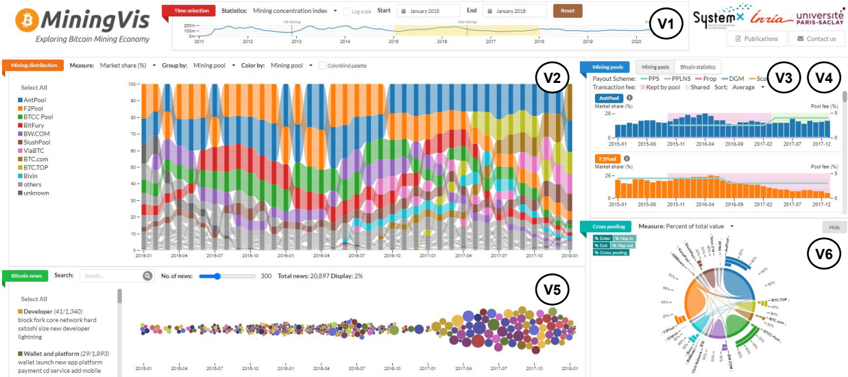
Fig. 1. A screenshot of the MiningVis tool. (V1) The time filter view allows analysts to select a time interval of interest. (V2) The mining distribution view shows the evolution of the mining pools as a ribbon chart. (V3) The mining pool details view shows mining power and pool characteristics for each mining pool in a compound chart. (V4) The Bitcoin statistics view shows Bitcoin network statistics as a list of area charts (see Fig. 4). (V5) The Bitcoin news view displays a swarm plot of the news distribution over time. (V6) The cross pooling view represents the total reward of cross pooling miners in mining pools at the time interval on a chord diagram.
