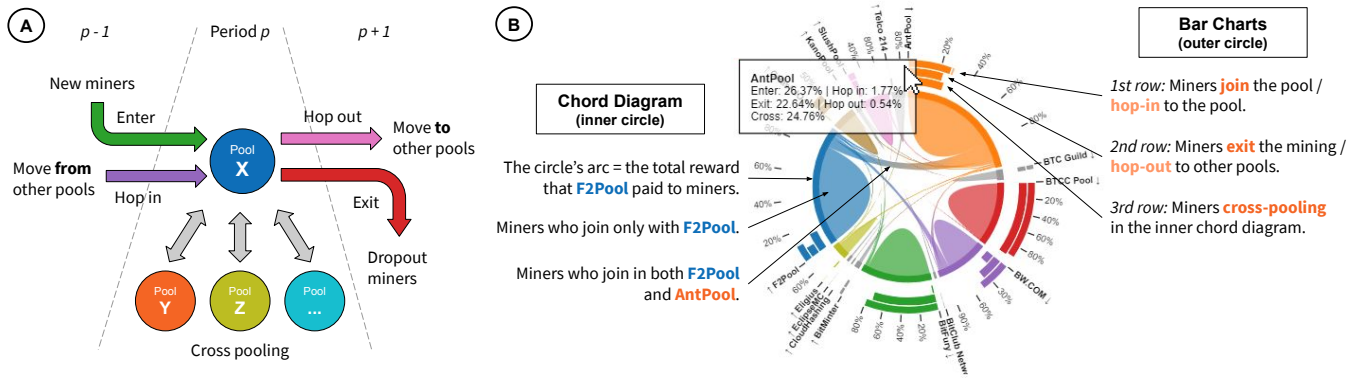
Fig. 6. The cross pooling view. (A) The stock and flow of miners’ migration in a mining pool. This is a simplified version of our previous miners’ migration flow model [62]. (B) Our visual representation of the miners’ migration flows as a chord diagram and bar charts. The economist observed the high cross-pooling between F2Pool and AntPool and detect both pools have the higher incoming miners than outgoing ones (in the bar chart).
