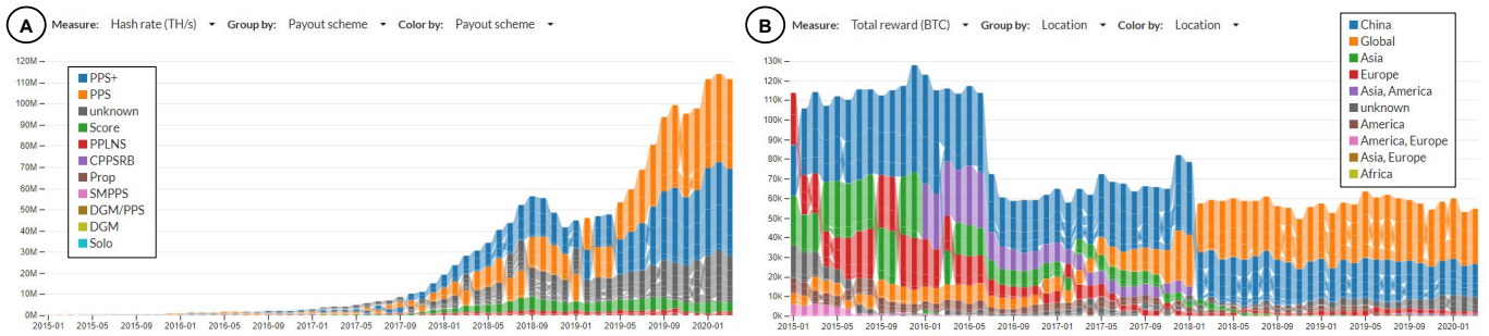
Fig. 2. The mining pool distribution view (V2) with different configurations. (A) Measure: Hash rate (TH/s), Grouped by: Payout scheme, and Color by: Payout scheme. The economist detected that the hash rate is growing while mining pools with the PPS payout scheme dominated in the market after Apr 2015. (B) Measure: Total reward, Grouped by: Location, Color by: Location. The economist detected the halving in rewards in July 2016 when Chinese pools dominated the market. After the local peak between Dec 2017–Jan 2018, global pools overtake Chinese pools in the market.
