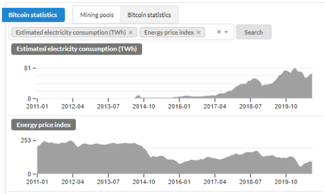
Fig. 4. The Bitcoin statistics view (V4) shows each Bitcoin statistics measure as the area chart. Analysts can browse the list of statistics measures and correlate with measures shown in V2.
