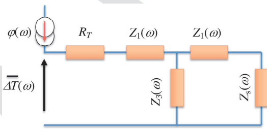
FIG. 9. Heat transfer model within the front face PPTR configuration considering the heat penetration depth is larger than the PCM thickness.
