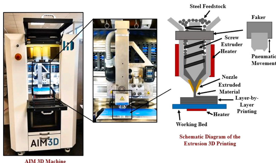
Fig. 3. Schematic diagram and picture of the Exam 255 3D printing machine from AIM3D™.
