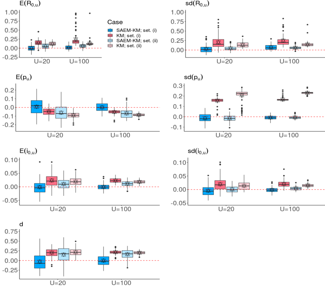
Fig. 3 Boxplots (25th, 50th and 75th percentiles) of the bias of the estimates of each model parameter, with \bar{n} = 50 , obtained with SAEM-KM (blue boxes) and KM (red boxes). Two levels: U = 20 and U = 100 epidemics. Dark colours: high inter-epidemic variability (setting (i)). Light colours: moderate inter-epidemic variability (setting (ii)). The symbol represents the estimated mean bias. For sake of clarity, we removed extreme values from the graphical representation. This concerns only the parameter R_0 and the KM method: 37 values for \mathbb{E}(R_{0,u}) (35 in setting (i), 2 in setting (ii)) and 50 values for \text{sd}(R_{0,u}) (47 in setting (i), 3 in setting (ii)).
