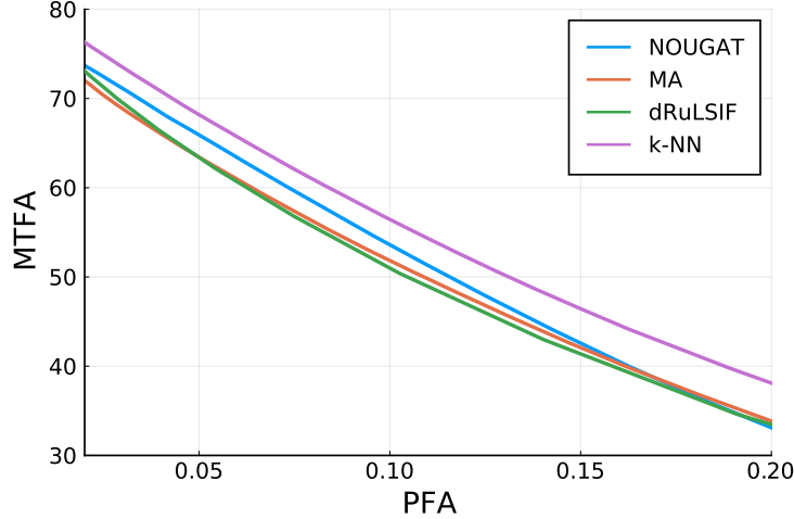
Figure 10: MTFA as a function of PFA for NOUGAT, MA and dRuLSIF.
