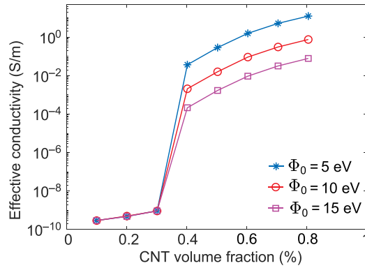
FIGURE 10 Effective conductivity versus CNT volume fraction for several barrier heights \Phi_0 , \bar{E}_x = 0.125 V/ \mu\text{m} , l/D = 100
