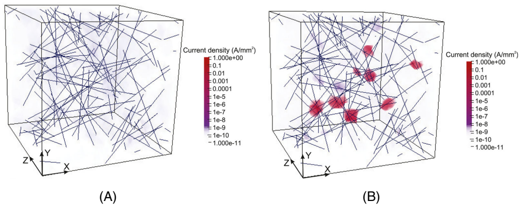
FIGURE 7 Current density in the polymer matrix of microstructure with CNT volume fraction f = 1.58 \text{ vol}\% , l/D = 40 . Side length of RVE L = 2.5 \mu\text{m} , \bar{E}_x = 0.125 \text{ V}/\mu\text{m} : (A) without tunneling effect; (B) considering tunneling effect. The values below the minimum of scale bar are set to transparency. The ParaView post-treatment software was used 70
