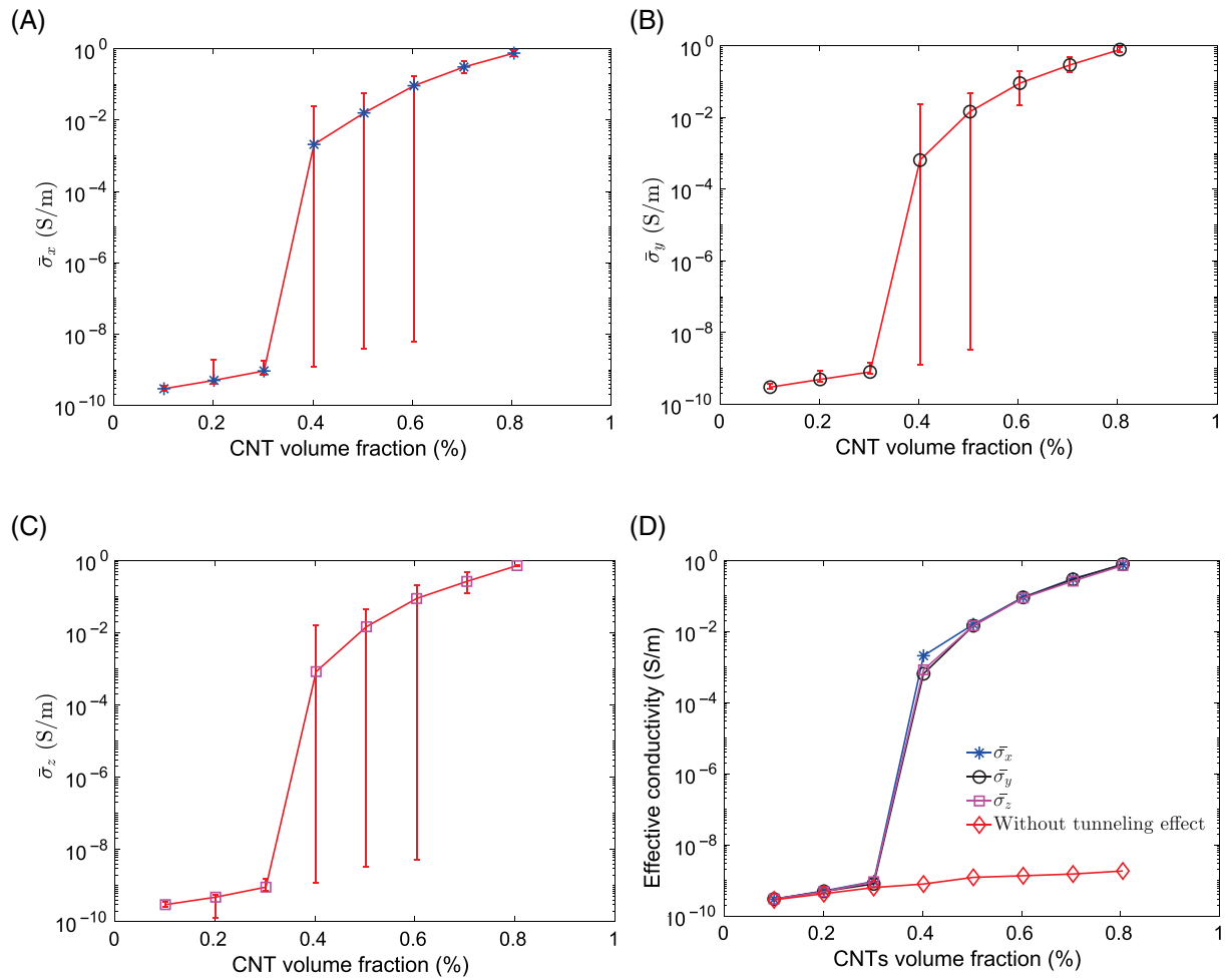
FIGURE 6 Effective conductivities tensor components (mean value and range) as a function of the CNT volume fraction, \bar{E} = 0.125 \text{ V}/\mu\text{m} , \Phi_0 = 10 \text{ eV} , l/D = 100 . (A) \bar{\sigma}_x , (B) \bar{\sigma}_y , (C) \bar{\sigma}_z , (D) Comparison with the case in which tunneling effect is neglected
