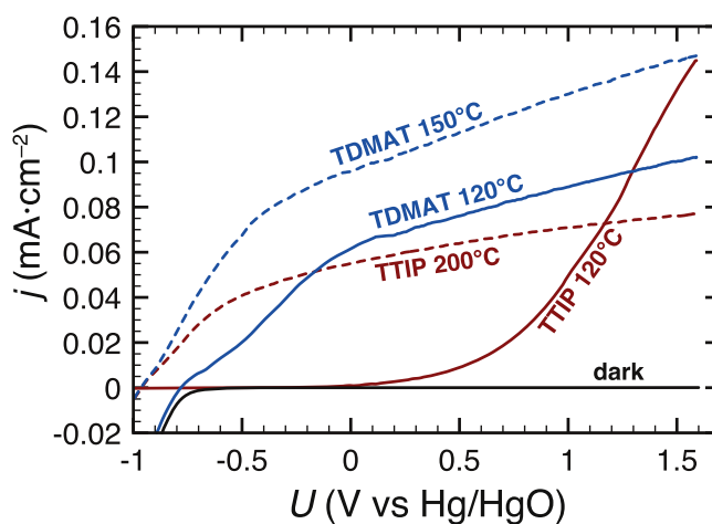
Figure 3. Linear sweep voltammograms of n-Si/ \text{TiO}_2 photoanodes in 1 M KOH under illumination ( P = 100\ \text{mW}\cdot\text{cm}^{-2} ). The 35 to 40 nm-thick \text{TiO}_2 films were grown using different Ti precursors (TTIP and TDMAT) at different T_{\text{ALD}} as indicated on the plot. A voltammogram measured in dark conditions is plotted as reference. The scan rate is 20\ \text{mV}\cdot\text{s}^{-1} .
