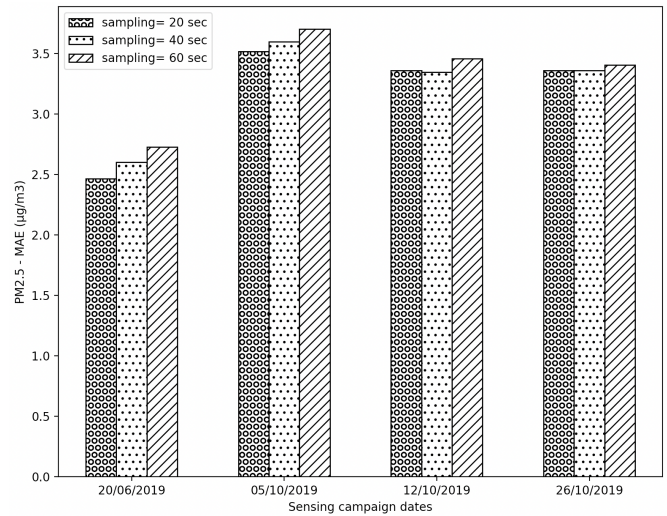
Fig. 4. MAE of PM_{2.5} concentrations estimation with three different sampling frequencies using 80% of data for training
