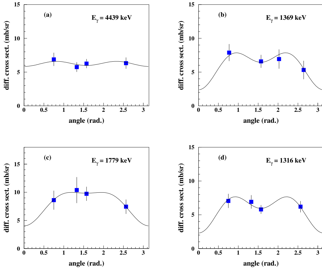
Figure 5: Examples of measured differential \gamma -ray emission cross sections (blue symbols) and Legendre-polynomial fits (black lines). Data from (a) irradiation of the C target at E_\alpha = 75 MeV, (b) irradiation of the Mg target at E_\alpha = 50 MeV, (c) irradiation of the Si target at E_\alpha = 60 MeV and (d) irradiation of the Fe at target E_\alpha = 90 MeV, the \gamma -ray line energies being indicated on the figures.
