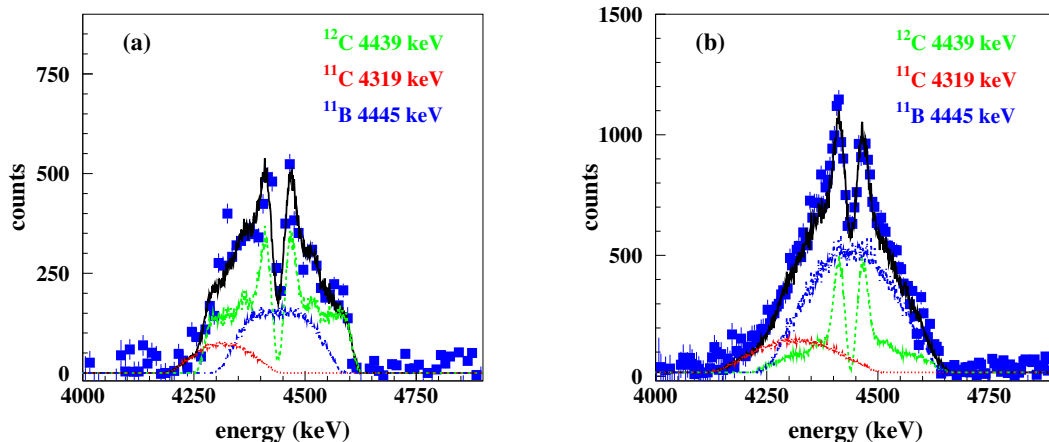
Figure 8: Symbols show the 4.44-MeV line complex in Compton-suppressed spectra of the Ge detectors sitting at \Theta = 90^\circ for (a) E_\alpha = 50 MeV and (b) E_\alpha = 75 MeV. The different lines show calculated line shapes for the 4439-keV line of ^{12}\text{C} from inelastic scattering (dashed green), the 4319-keV line of ^{11}\text{C} (dotted red) and the 4445-keV line of ^{11}\text{B} (dot-dashed blue), the solid black line showing the sum of the calculated lines. Inelastic scattering off ^{12}\text{C} accounts here to about 60% and 30% of the line complex at E_\alpha = 50 MeV and 75 MeV, respectively.
