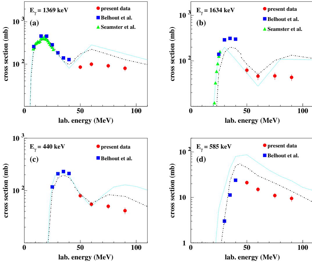
Figure 12: Symbols show measured cross section data for four different lines emitted in \alpha -particle reactions with natural Mg target from the present experiment, and with enriched ^{24}\text{Mg} targets from Belhout et al. [4] and Seamster et al. [21]. \gamma -ray line energies indicated in the panels refer to the lines listed in Table 5. The dotted cyan lines show the values from the cross-section compilation [14] and the dot-dashed black lines are the results of TALYS calculations. TALYS cross sections up to 45 MeV are the results for a ^{24}\text{Mg} target, and above 45 MeV for a natural Mg target.
