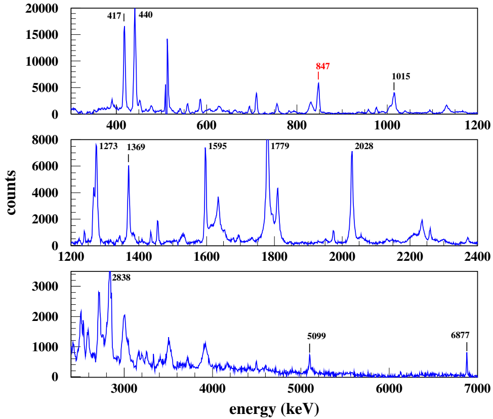
Figure 13: Compton-suppressed spectrum of the HP-Ge detector at \Theta = 90^\circ from the irradiation of the Si target with 60-MeV \alpha particles in the 2016 experiment in 1-keV/channel resolution below 2.4 MeV and 5-keV/channel resolution above. A selection of lines listed in table 6 are marked with their energy in keV, as well as the 847-keV line of ^{56}\text{Fe} line produced in interactions of secondary particles in the chamber walls and tubes.
