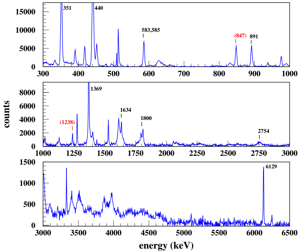
Figure 10: Compton-suppressed spectrum of the HP-Ge detector at \Theta = 90^\circ from the irradiation of the Mg target with 60-MeV \alpha particles in the 2016 experiment in 1-keV/channel resolution below 3 MeV and 5-keV/channel resolution above. A selection of strong lines listed in table 5 are marked with their energy in keV, as well as lines due to interactions of secondary particles in the chamber walls and tubes (red numbers in parenthesis).
