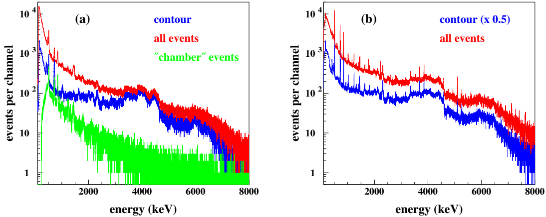
Figure 3: \gamma -ray spectra recorded by the LaBr 3 at \Theta = 76^\circ (a) and the HP-Ge detector at \Theta = 90^\circ (b) during irradiation of the carbon target by a 60-MeV \alpha -particle beam in the 2016 campaign. The blue lines show the spectra for events selected by the contour around the prompt \gamma rays from the target (see Fig. 2), red lines are the spectra for all events with energy and timing signal. The green line for the LaBr 3 detector are events dominated by interactions of secondary particles in the target chamber walls and tubes.
