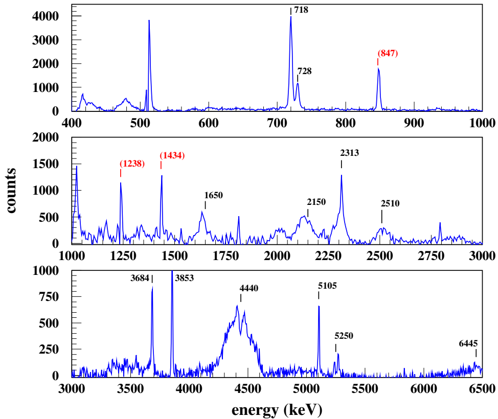
Figure 6: Compton-suppressed spectrum of the HP-Ge detector at \Theta = 90^\circ from the irradiation of the C target with 60-MeV \alpha particles in the 2016 experiment with 1-keV/channel resolution below 1 MeV and 5-keV/channel resolution above. The lines listed in table 4 are marked with their energy in keV, as well as lines due to interactions of secondary particles in the chamber walls and tubes (red numbers in parenthesis).
