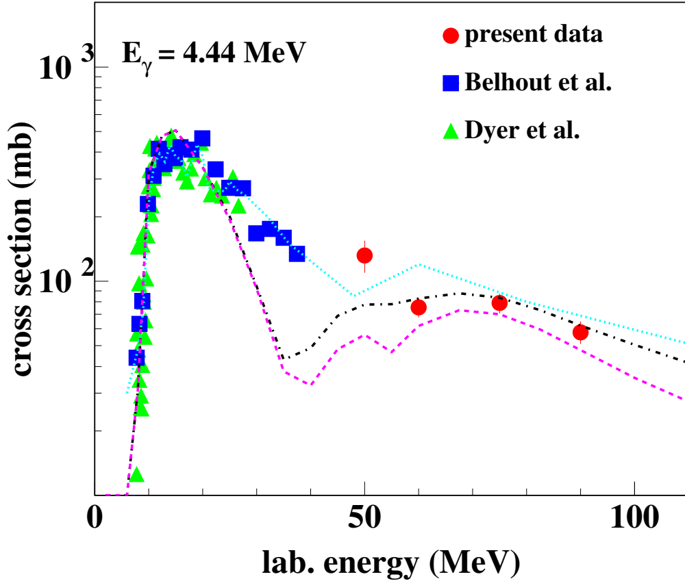
Figure 7: Cross section for emission of the 4.44-MeV line in \alpha -particle reactions with natural carbon targets in the present experiment and in Belhout et al. [4] and with enriched ^{12}\text{C} targets in Dyer et al. [9]. The dotted cyan line shows the values of the MKKS compilation [14], the dot-dashed black line is the result of calculations with the TALYS-1.6 code [11] with default parameters, including \gamma -ray lines in the window E_\gamma = 4439 \pm 140 \text{ keV} , while the dashed magenta line shows the contribution of the 4439-keV line of ^{12}\text{C} .
