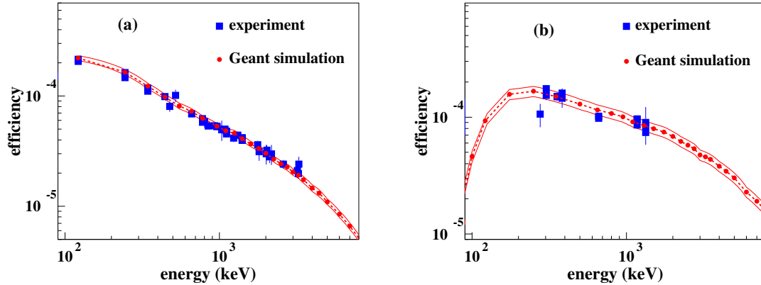
Figure 1: Full-energy-peak detection efficiencies of HP-Ge detectors at 90^\circ in the 2015 (a) and the 2016 campaign (b). Measured efficiency data with radioactive sources in the target chamber are shown by blue squares and simulated ones by red circles, connected with the dashed curve. The red upper and lower lines enclosing the simulation efficiencies represent the adopted uncertainty for the detection efficiency. For the HP-Ge detector in 2015, additionally to the standard radioactive sources, data from the decay of ^{55}\text{Co} and ^{56}\text{Co} in the activated beam dump could be obtained.
