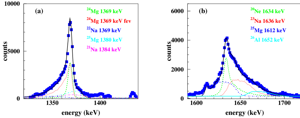
Figure 11: Symbols show (a) the 1.37-MeV line complex in Compton-suppressed spectra of the Ge detectors sitting at \Theta = 147^\circ for E_\alpha = 75 MeV and (b) the 1.63-MeV line complex at \Theta = 43^\circ for E_\alpha = 60 MeV. The dashed, dotted and dot-dashed lines show calculated line shapes for the strongest components. The sum of all components is shown by the solid black lines. Two separated calculations were done for the 1369-keV line of ^{24}\text{Mg} , one for the inelasting scattering component and one for the fusion-evaporation component, labelled "fev" in (a).
