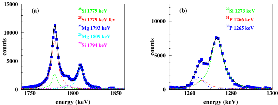
Figure 14: Symbols show (a) the 1.78-MeV and (b) the 1.27-MeV line complexes in Compton-suppressed spectra of the Ge detector sitting at \Theta = 90^\circ for E_\alpha = 60 MeV. The dashed, dotted and dot-dashed lines show calculated line shapes for the strongest components. The sum of all components is shown by the solid black lines. Two separated calculations were done for the 1779-keV line of ^{28}\text{Si} , one for the inelasting scattering component and one for the fusion-evaporation component, labelled "fev" in (a).
