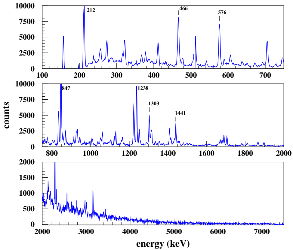
Figure 16: Compton-suppressed spectrum of the HP-Ge detector at \Theta = 90^\circ from the irradiation of the Fe target with 60-MeV \alpha particles in the 2016 experiment in 1-keV/channel resolution below 2.0 MeV and 5-keV/channel resolution above. A selection of lines listed in table 7 are marked with their energy in keV.
