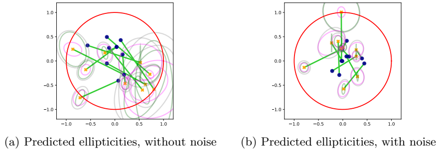
Fig. 9. Predicted ellipticities on the complex plane for blended galaxies images. In red: unit circle. In yellow: predicted ellipticities. In blue: target ellipticities (label of the centered galaxy). In light green: difference between true and predicted values. In pink: 90% epistemic confidence ellipse. In dark green: 90% aleatoric confidence ellipse. In grey: 90% predictive confidence ellipse
