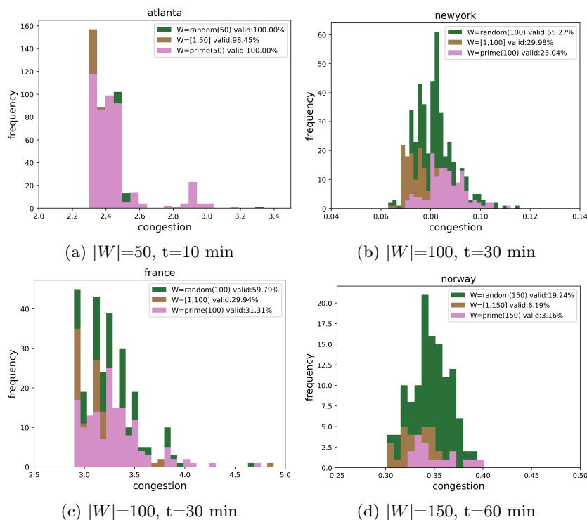
Fig. 3. Distribution of the congestion values with different metric spaces of the same size using NRPA with force_exploration
