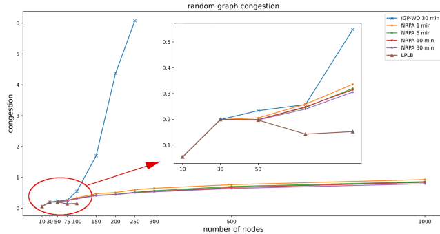
Fig. 6. Congestion with respect to the number of the nodes
