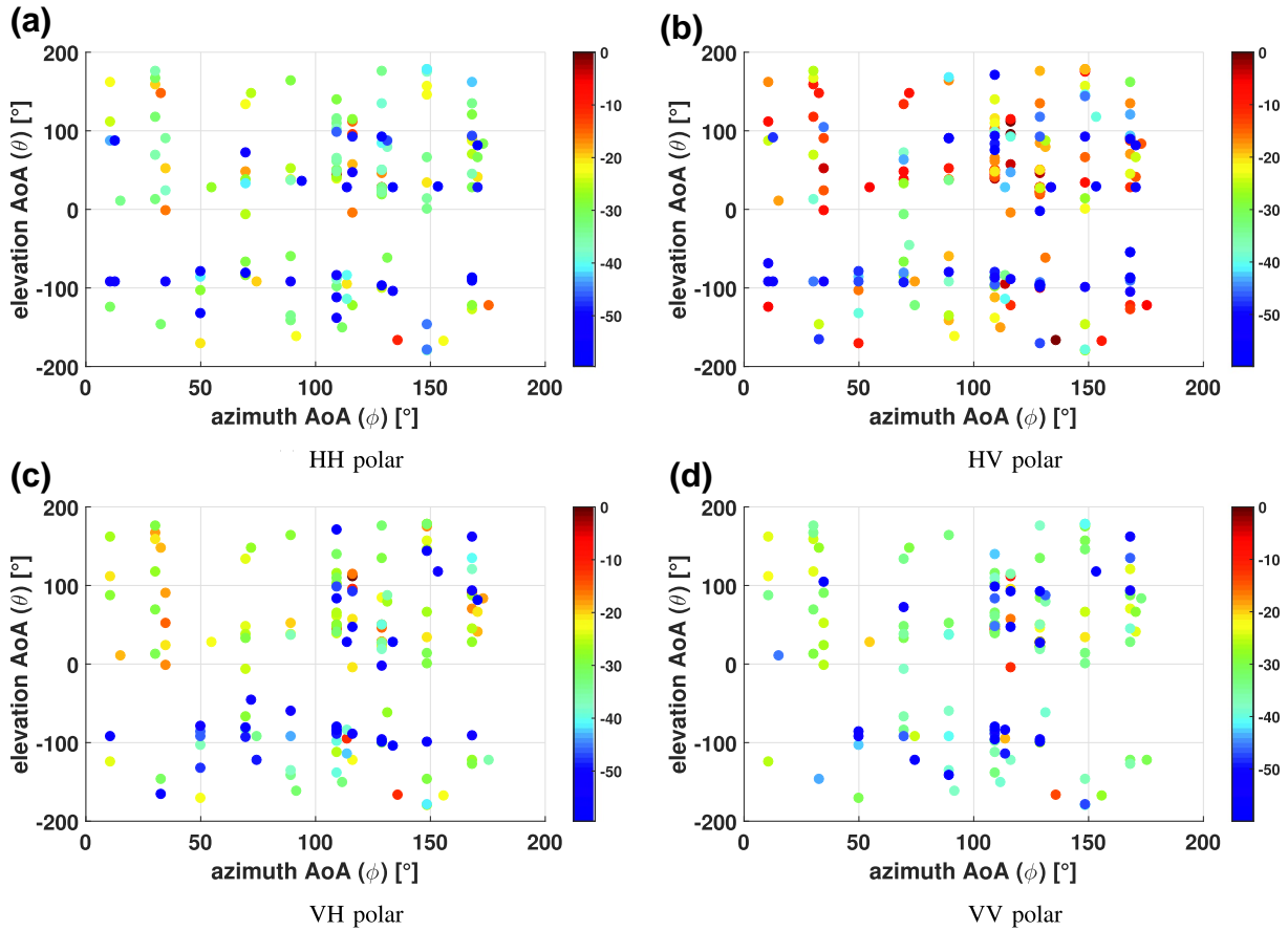
FIGURE 2 Multipath parameters at Position 1 (LOS conditions). LOS, line-of-sight
