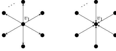
Fig. 4 An out-star graph S and an in-star graph T .
