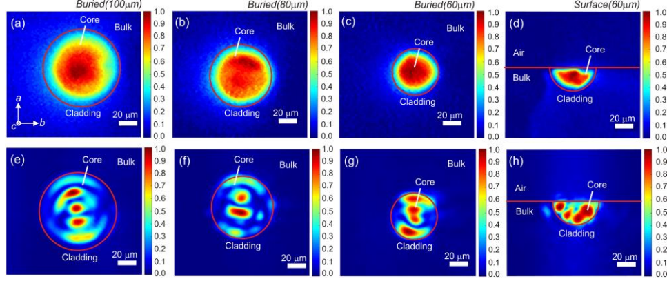
Fig. 8. Near-field pump modes for depressed-index fs-DLW channel WGs in Tm:CALGO: top row: (a)-(c) \lambda_p = 798 nm, bottom row: (e)-(f) \lambda_p = 1679 nm; buried WGs with a circular cladding and a diameter of (a,e) 100 \mu\text{m} , (b,f) 80 \mu\text{m} , (c,g) 60 \mu\text{m} and (d,h) surface WG with a half-ring cladding (size: 60 \mu\text{m} ). The red circular lines indicate the cladding / crystal surface and are drawn as a guide for the reader.
