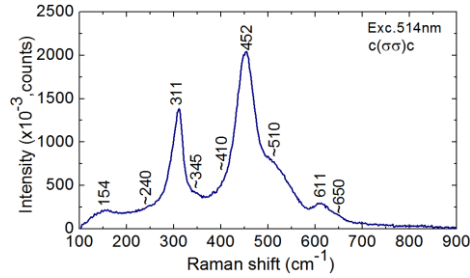
Fig. 5. Raman spectrum of the c -cut Tm:CALGO bulk crystal. The measurement geometry is c(\sigma\sigma)c , \lambda_{\text{exc}} = 514 nm. The numbers indicate the Raman frequencies in \text{cm}^{-1} .
