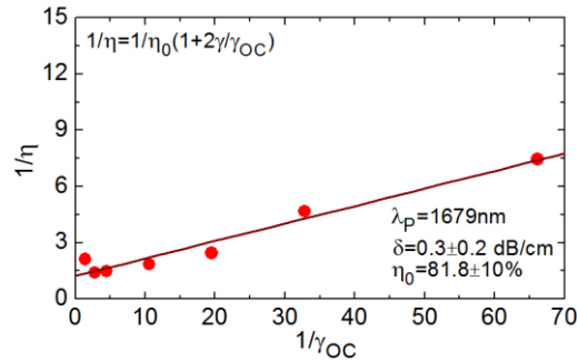
Fig. 12. Caird analysis of intracavity losses in the in-band pumped \text{Tm} :CALGO buried WG laser (circular cladding with a diameter of 60 \mu\text{m} ): inverse of the slope efficiency, 1/\eta , vs. inverse of the output-coupling loss, 1/\gamma_{OC} , circles – experimental data, line – their fit.
