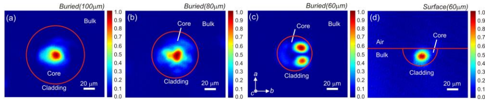
Fig. 13. Near-field profiles of the laser mode for in-band pumped \text{Tm} :CALGO WG lasers: (a)–(c) buried WGs with a circular cladding (diameter: (a) 100 \mu\text{m} , (b) 80 \mu\text{m} , (c) 60 \mu\text{m} ); (d) surface WG with a half-ring cladding (size: 60 \mu\text{m} ). The red circular lines indicate the cladding / crystal surface and are drawn as a guide for the reader. T_{OC} = 20\% .
