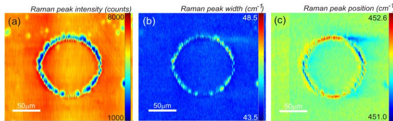
Fig. 6. \mu -Raman mapping of a depressed-index buried channel WG with a circular cladding (size: 100 \mu\text{m} ) fabricated in a Tm:CALGO crystal by fs-DLW: (a) peak intensity, (b) width (FWHM), (c) position; monitoring the \sim 452 \text{cm}^{-1} mode in the c(\sigma\sigma)c geometry, \lambda_{\text{exc}} = 514 nm.
