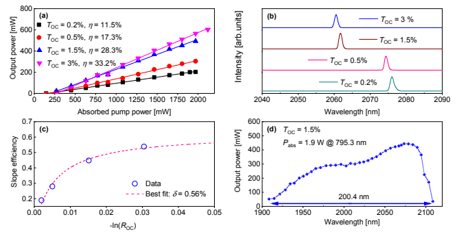
Fig. 2. CW laser performance of the mixed Tm:LuY 2 O 3 ceramic for different OCs (a); laser spectra (b); slope efficiency as a function of the OC reflectivity R_{OC} = 1 - T_{OC} (c); and spectral tuning range obtained with a Lyot filter (d).
