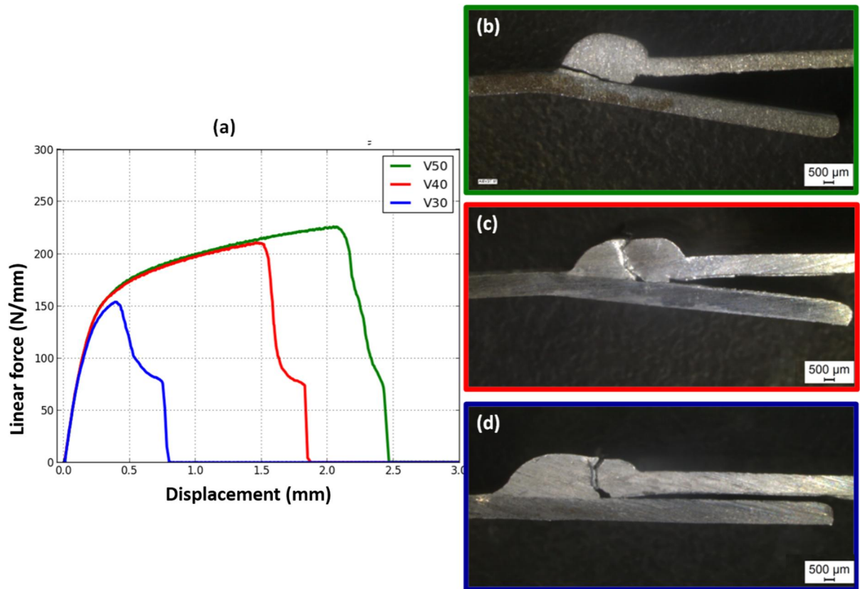
Fig. 10. (a) Tensile curves, and fracture location in assemblies made with welding speed of (b): 50 \text{ cm.min}^{-1} , (c): 40 \text{ cm.min}^{-1} , (d): 30 \text{ cm.min}^{-1} .
