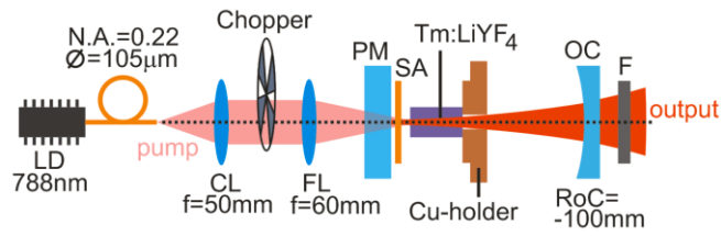
Figure 1. Scheme of the diode-pumped Tm:LiYF 4 laser Q-switched by the Cr 2+ :ZnSe SA: LD – laser diode, CL and FL – collimating and focusing lens, respectively, PM – pump mirror, SA – saturable absorber, OC – output coupler, F – cut-off filter.
