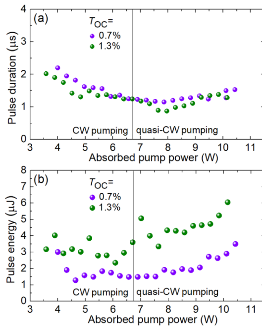
Figure 5. Pulse characteristics: (a) duration (FWHM) and (b) energy for the diode-pumped \text{Tm}:\text{LiYF}_4 laser PQS by a \text{Cr}^{2+}:\text{ZnSe} SA.
