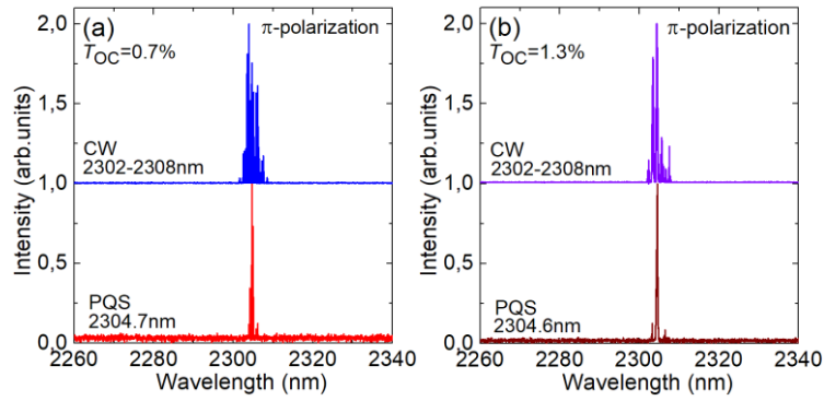
Figure 4. Typical spectra of laser emission for the CW and \text{Cr}^{2+}:\text{ZnSe} PQS diode-pumped \text{Tm}:\text{LiYF}_4 lasers: (a) T_{\text{OC}} = 0.7\% , (b) T_{\text{OC}} = 1.3\% . P_{\text{abs}} \sim 6 \text{ W} . The laser polarization is \pi .
