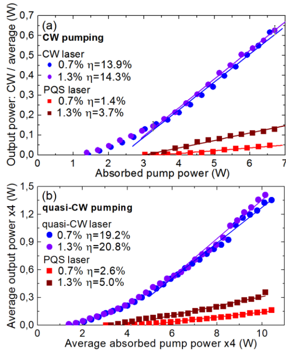
Figure 3. Input-output dependences for the CW and Cr 2+ :ZnSe PQS diode-pumped Tm:LiYF 4 lasers: (a) CW pumping, (b) quasi-CW pumping (duty cycle: 1:4), \eta – slope efficiency.
