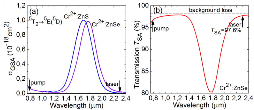
Figure 2. Saturable absorber: (a) Ground-state absorption cross-sections, \sigma_{GSA} , for Cr 2+ ions in ZnS and ZnSe materials; (b) Small-signal intrinsic transmission ( T_{SA} ) spectrum (subtracting the effect from the coatings) of the Cr 2+ :ZnSe SA ( t = 1.0 mm). The arrows in (a,b) indicate the pump (0.79 \mu\text{m} ) and laser (2.30 \mu\text{m} ) wavelengths.
