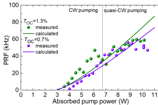
Figure 6. Pulse repetition frequency for the diode-pumped \text{Tm}:\text{LiYF}_4 laser PQS by a \text{Cr}^{2+}:\text{ZnSe} SA: symbols – experimental data, curves – modelling.
