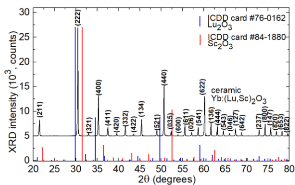
Fig. 3. X-ray powder diffraction pattern of 10 at.% Yb:(Lu,Sc) 2 O 3 ceramics, red and blue peaks – theoretical patterns for Lu 2 O 3 (ICDD card #76-0162) and Sc 2 O 3 (ICDD card #84-1880), numbers – Miller's indices ( hkl ).
