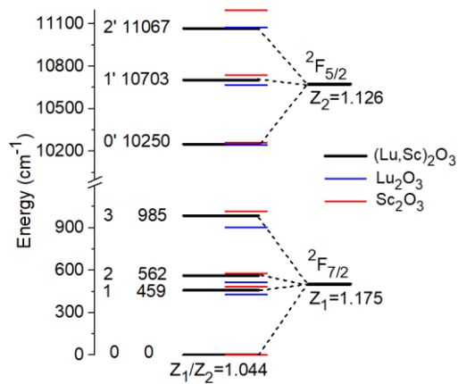
Fig. 10. Crystal-field splitting of \text{Yb}^{3+} ions in \text{C}_2 sites in the (\text{Lu,Sc})_2\text{O}_3 ceramics, Stark splitting for \text{Lu}_2\text{O}_3 and \text{Sc}_2\text{O}_3 are given for comparison.
