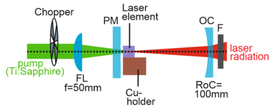
Fig. 11. Scheme of the laser set-up: FL – focusing lens, PM – pump mirror, OC – output coupler, F – cut-on filter.
