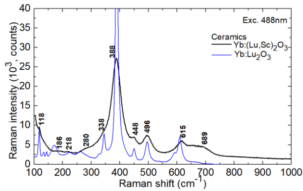
Fig. 4. RT Raman spectrum of \text{Yb:(Lu,Sc)}_2\text{O}_3 ceramics. The spectrum for \text{Yb:Lu}_2\text{O}_3 is shown for comparison, numbers – peak Raman frequencies, \lambda_{\text{exc}} = 488 \text{ nm} .
