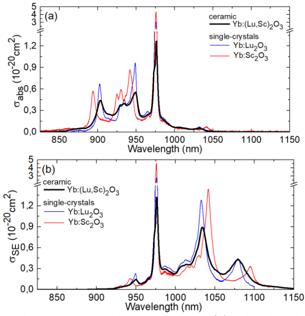
Fig. 6. (a) Absorption cross-sections, \sigma_{\text{abs}} , and (b) stimulated-emission cross-sections, \sigma_{\text{SE}} , for the {}^2F_{7/2} \leftrightarrow {}^2F_{5/2} \text{Yb}^{3+} transition in (\text{Lu,Sc})_2\text{O}_3 ceramics at RT. The spectra for bulk \text{Yb:Lu}_2\text{O}_3 and \text{Yb:Sc}_2\text{O}_3 crystals are given for comparison.
