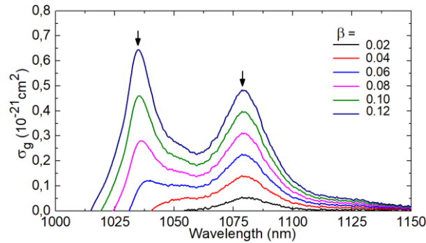
Fig. 7. RT gain cross-sections, \sigma_g = \beta\sigma_{\text{SE}} - (1 - \beta)\sigma_{\text{abs}} , for the {}^2F_{7/2} \leftrightarrow {}^2F_{5/2} \text{Yb}^{3+} transition in (\text{Lu,Sc})_2\text{O}_3 ceramics for different inversion ratios \beta = N_2({}^2F_{5/2})/N_{\text{Yb}} , arrows indicate the observed laser wavelengths.
