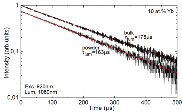
Fig. 8. RT luminescence decay curve for the 10 at.% Yb:(Lu,Sc) 2 O 3 ceramics (bulk and powdered samples), \lambda_{\text{exc}} = 920 \text{ nm} , \lambda_{\text{lum}} = 1080 \text{ nm} , lines – single-exponential fits.
