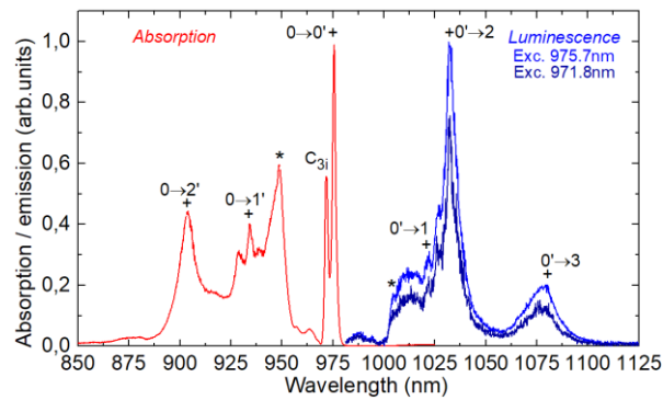
Fig. 9. LT (12 K) absorption and luminescence spectra for the Yb:(Lu,Sc) 2 O 3 ceramics, \lambda_{\text{exc}} = 975.7 and 971.8 \text{ nm} , the symbol “+” refers to electronic transitions of Yb 3+ ions in C 2 sites, asterisks refer to the assignment from Ref. [34].
