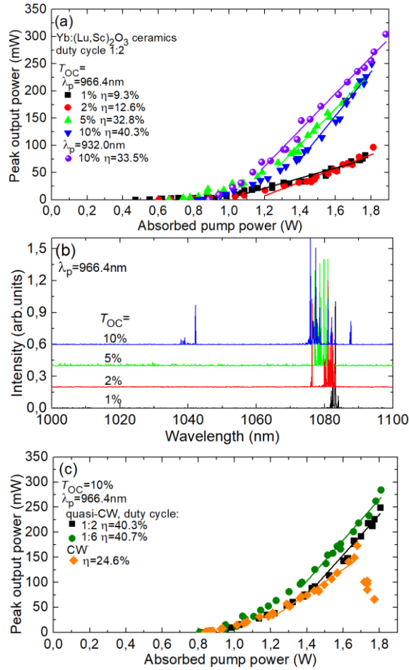
Fig. 12. 10 at.% Yb:(Lu,Sc) 2 O 3 ceramic laser: (a) input-output dependences, \eta – slope efficiency, (b) typical spectra of laser emission captured at P_{abs} \sim 1.6\text{ W} , \lambda_p = 966.4\text{ nm} . Quasi-CW pumping, duty cycle: 1:2; (c) Comparison of CW and quasi-CW laser performance for T_{OC} = 10\% , \lambda_p = 966.4\text{ nm} .
