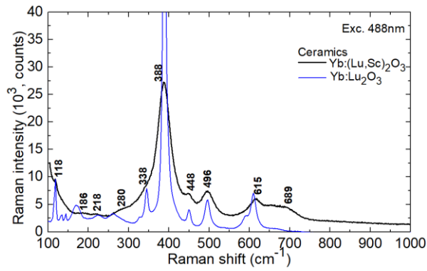
Fig. 4. RT Raman spectrum of \text{Yb}:(\text{Lu},\text{Sc})_2\text{O}_3 ceramics. The spectrum for \text{Yb}:\text{Lu}_2\text{O}_3 is shown for comparison, numbers – peak Raman frequencies, \lambda_{\text{exc}} = 488 \text{ nm} .
