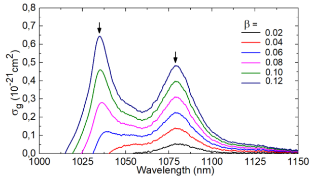
Fig. 7. RT gain cross-sections, \sigma_g = \beta\sigma_{\text{SE}} - (1 - \beta)\sigma_{\text{abs}} , for the {}^2F_{7/2} \leftrightarrow {}^2F_{5/2} \text{Yb}^{3+} transition in (\text{Lu},\text{Sc})_2\text{O}_3 ceramics for different inversion ratios \beta = N_2({}^2F_{5/2})/N_{\text{Yb}} , arrows indicate the observed laser wavelengths.
