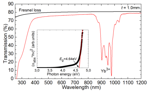
Fig. 5. Transmission spectrum of a laser-grade-polished \text{Yb}:(\text{Lu},\text{Sc})_2\text{O}_3 ceramic disk (thickness, t = 1.0 \text{ mm} ), black curve – theoretical transmission determined by the Fresnel losses for (\text{Lu}_{2/3}\text{Sc}_{1/3})_2\text{O}_3 . Inset – Tauc plot for determination of the optical bandgap E_g (assuming direct transitions).
