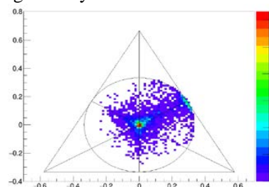
Figure 1. Dalitz plot obtained for the fragmentation of (\text{CO})_3^{3+} in three singly charged (\text{CO})^+ fragments.
