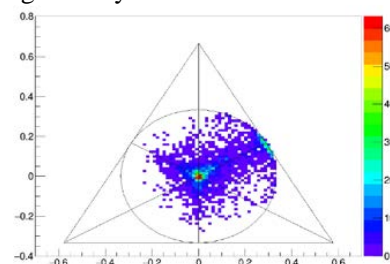
Figure 1. Dalitz plot obtained for the fragmentation of (\text{CO})_3^{3+} in three singly charged (\text{CO})^+ fragments.
