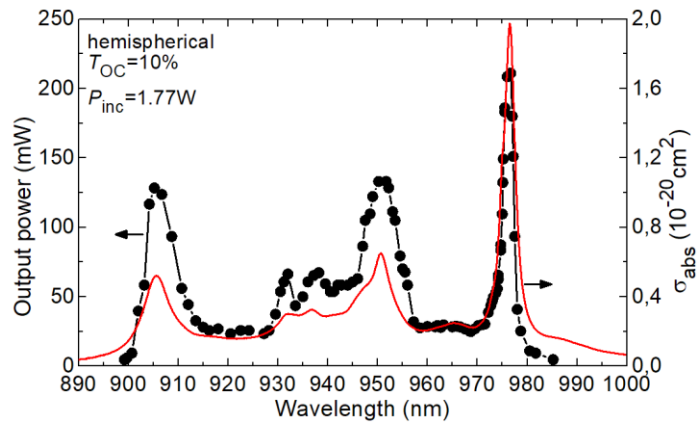
Figure 12. Laser excitation curve (output power vs. the pump wavelength) for the 2 at.% Yb:Y 2 O 3 ceramic laser, T_{OC} = 10\% , P_{inc} = 1.77 W. The \sigma_{abs} spectrum for Yb 3+ ions is shown for comparison.
