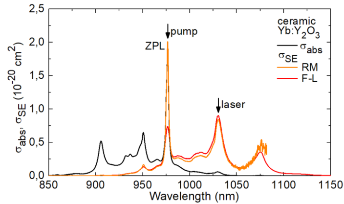
Figure 7. Absorption, \sigma_{abs} , and stimulated-emission (SE), \sigma_{SE} , cross-sections for the {}^2F_{7/2} \leftrightarrow {}^2F_{5/2} transition of Yb^{3+} ions in the 2 at.% Yb:Y_2O_3 ceramics fabricated using LiF sintering additive. Arrows indicate the pump and laser wavelengths.
