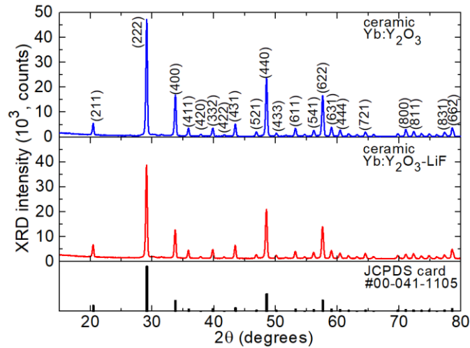
Figure 6. X-ray powder diffraction patterns of 2 at.% Yb:Y 2 O 3 ceramics prepared from Yb:Y 2 O 3 and Yb:Y 2 O 3 – LiF nanopowders.
