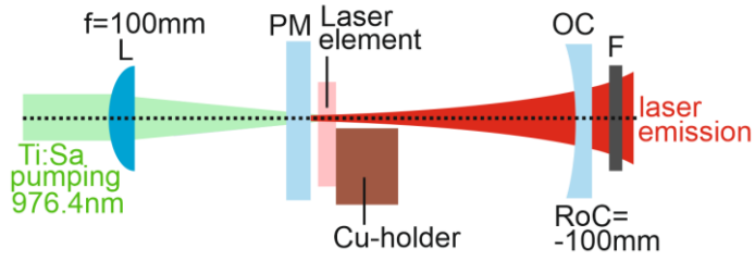
Figure 10. Scheme of the laser set-up: L – focusing lens, PM – pump mirror, OC – output coupler, F – long-pass filter.
