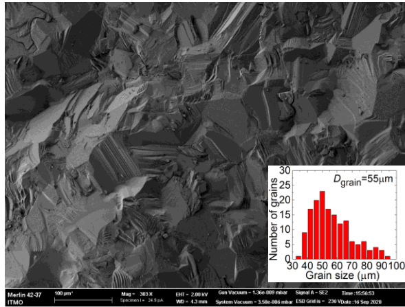
Figure 5. SEM image of the fractured surface of Yb:Y 2 O 3 ceramic fabricated from Yb:Y 2 O 3 – LiF nanopowders, after HIPing, inset – typical grain size distribution.
