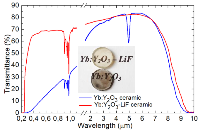
Figure 4. Transmission spectra of hot-pressed ceramics fabricated from \text{Yb:Y}_2\text{O}_3 and \text{Yb:Y}_2\text{O}_3 - \text{LiF} nanopowders, inset – photographs of the as-sintered and polished ceramic disks.
