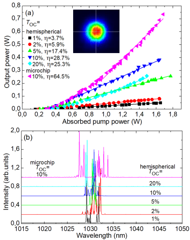
Figure 11. 2 at.% Yb:Y 2 O 3 ceramic laser: (a) input-output dependences, \eta – slope efficiency, inset – typical profile of the laser mode in the far-field, hemispherical cavity, T_{OC} = 10\% , P_{abs} \sim 1.0 W; (b) spectra of the laser emission at an absorbed pump power of 1.2 W, \lambda_P = 976.4 nm.
