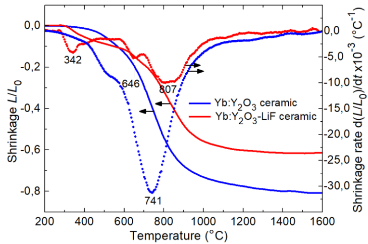
Figure 3. Shrinkage curves ( solid ) and shrinkage rate ( symbols ) of \text{Yb:Y}_2\text{O}_3 and \text{Yb:Y}_2\text{O}_3 - \text{LiF} green bodies.
