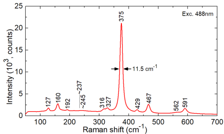
Figure 9. RT Raman spectrum of the 2 at.% Yb:Y_2O_3 ceramic fabricated using LiF sintering additive, numbers denote the Raman frequencies in cm^{-1} , \lambda_{exc} = 488 nm.
