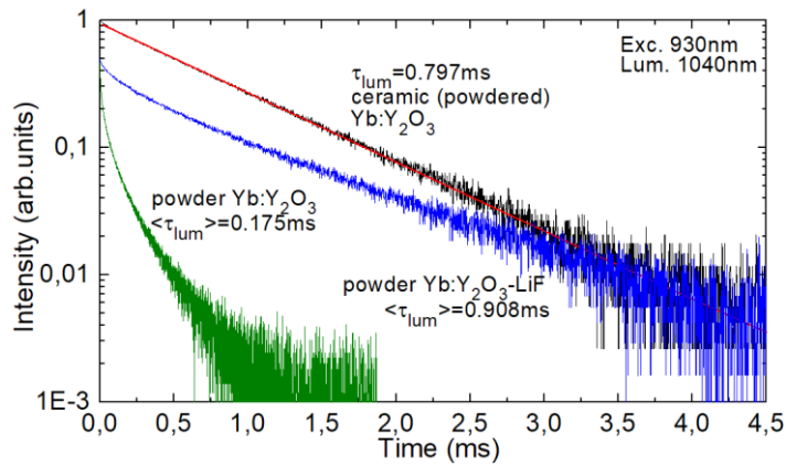
Figure 8. RT luminescence decay curves for Yb^{3+} ions in the Y_2O_3 ceramic fabricated using LiF sintering additive (powdered sample), Y_2O_3 and Y_2O_3 – LiF nanopowders, \lambda_{exc} = 930 nm, \lambda_{lum} = 1040 nm, \tau_{lum} – decay time.
