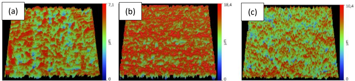
Figure 7. Topographies of surfaces tested prior to friction: (a) PMr1, (b) PMr2, and (c) RPa1.
