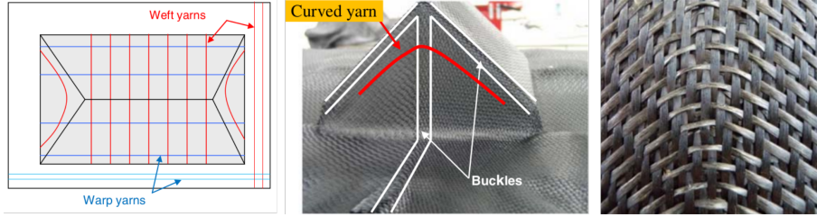
Figure 3: In-plane bending of fibers during a forming on a prism shape (Allaoui et al., 2014)
