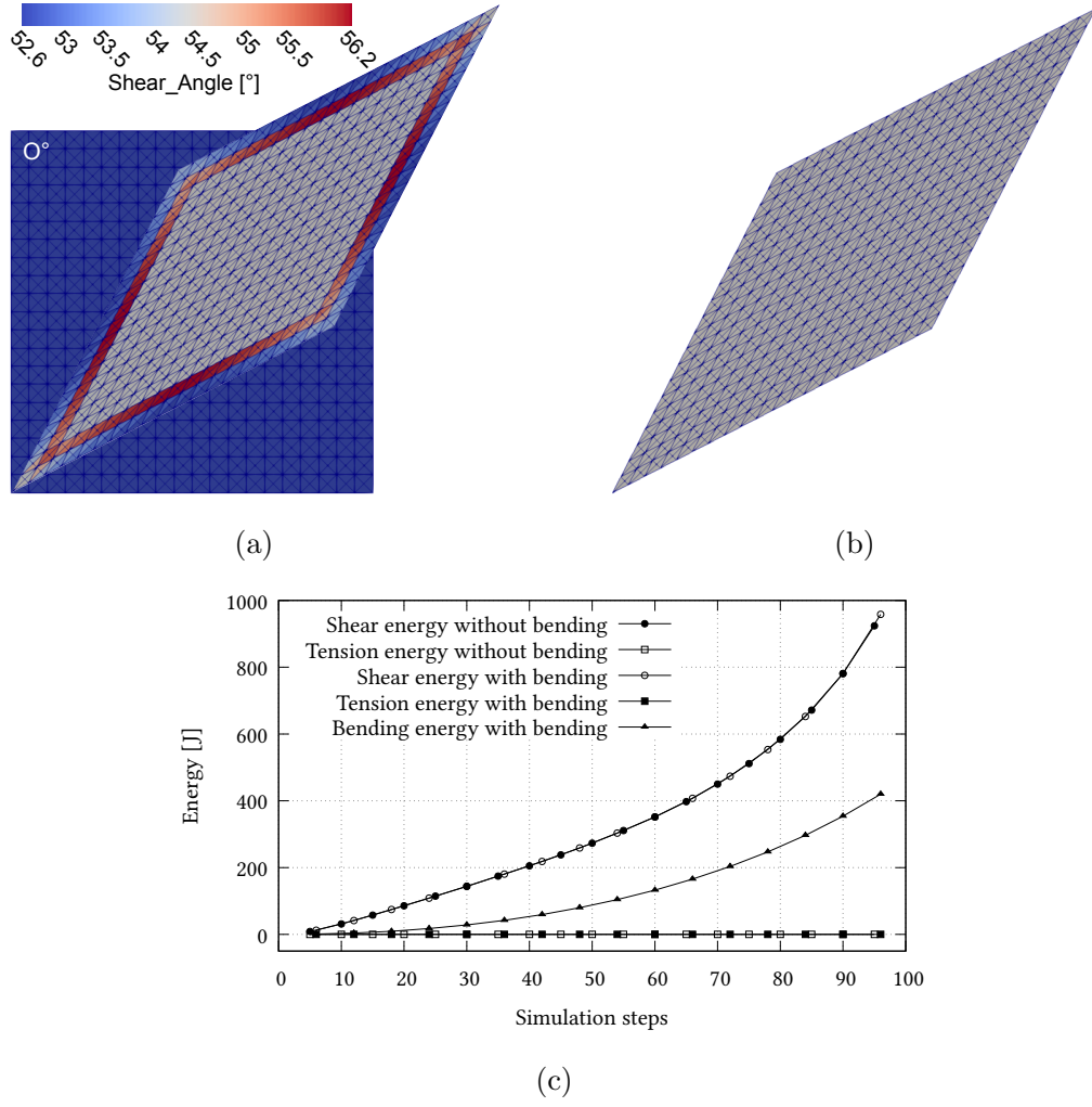
Figure 11: Picture frame simulation. (a) shear angle distribution accounting for in-plane bending rigidity; (b) shear angle distribution without in-plane bending rigidity (same color scale); (c) energetic contributions of tension, bending and shearing modes, with and without bending rigidity.
