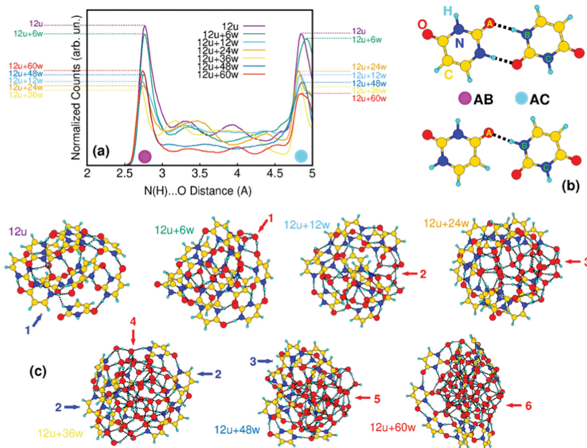
Fig. 4 (a) Normalized distributions of inter-uracil ( \text{N(H)}\cdots\text{O}=\text{C} ) distances averaged along 0.5 ns of molecular dynamics simulations of mixed clusters containing 12-uracil molecules and variable amounts (0–60) of water molecules. (b) Most relevant interaction patterns between uracil molecules, represented by bidirectional (upper) and monodirectional (lower) ( \text{N(H)}\cdots\text{O}=\text{C} ) hydrogen bonds; AB and AC distances represent the main peaks of panel (a). (c) Most stable structures found by applying the CREST algorithm in the investigated 12\text{u} + n\text{w} mixed cluster. Blue and red arrows refer to the evolution of water and uracil connectivity along the structures, as discussed in the text.
