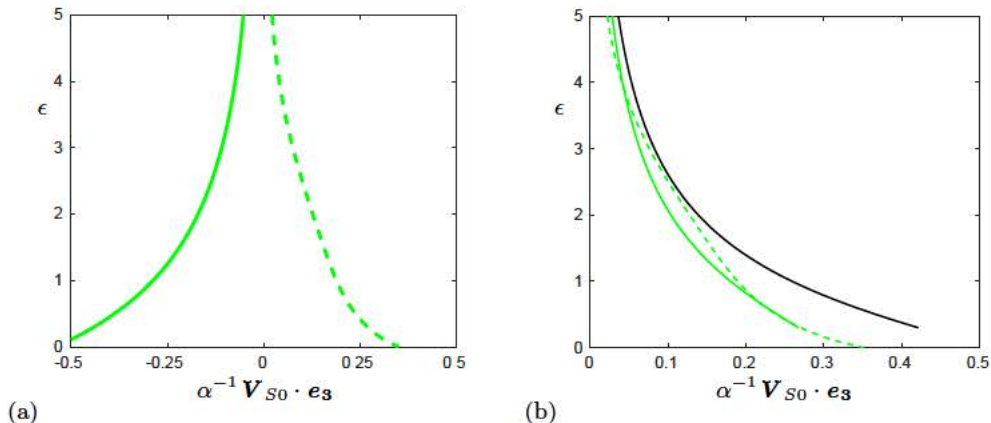
Figure 3: Slip velocity profile as a function of the gap \epsilon = \kappa^{-1} - 1 for a particle with relative radius \Delta^{-1} = 0.3 compared to the characteristic boundary layer thickness. (a) Comparison between simulation results (---) and predictions of the GMR equation using the undisturbed flow (2.2) with k_\delta = 1 (—); (b) comparison between simulation results (---) and predictions of (3.6) with k_\delta = 2 (—) and k_\delta = 1 (—).
