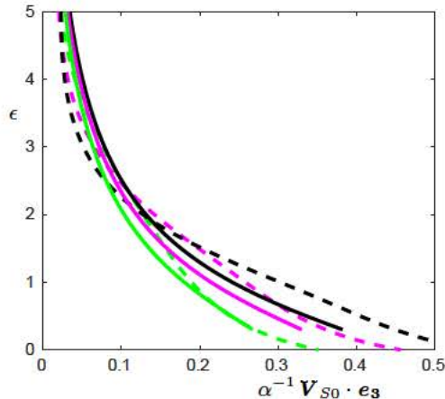
Figure 4: Slip velocity in the near-wall region for particles with increasing relative size \Delta^{-1} = 0.3 (—), 0.4 (—), 0.5 (—). Dashed line: simulation results; thin solid line: creeping-flow prediction (3.6) using the undisturbed flow (2.2) with k_\delta = 1 .
