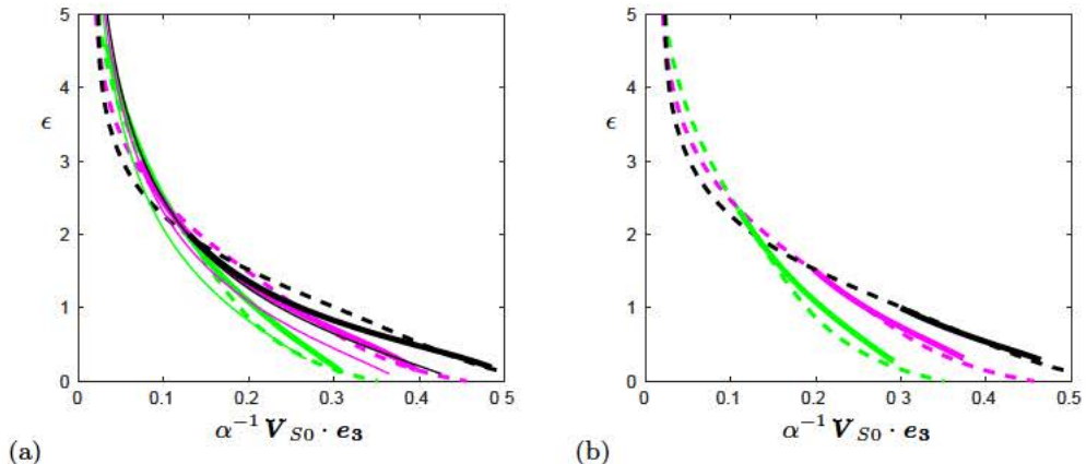
Figure 5: Predictions for the slip velocity in the near-wall region for particles with increasing relative size \Delta^{-1} = 0.3 (—), 0.4 (—), 0.5 (—); all predictions are based on the undisturbed flow (2.2) with k_\delta = 1 . (a): initial gap \epsilon_i = 3\Delta/2 - 1 ; (b): \epsilon_i = \Delta - 1 . Dashed line: simulation results; thick solid line: finite- Re prediction from (4.10); thin solid line in (a): creeping-flow prediction (3.6) (the thick purple line and the thin black line almost overlap).
