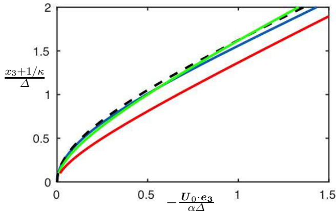
Figure 2: Near-wall profile of the wall-normal velocity in the base flow; the velocity and distance to the wall are normalized using boundary layer quantities, i.e. B\delta/V_c = \alpha\Delta and \delta/a = \Delta , respectively. Blue line: theoretical solution (Homann 1936); dotted line: numerical solution (Li et al. 2020); red and green lines: model (2.2) with k_\delta = 2 and k_\delta = 1 , respectively.
