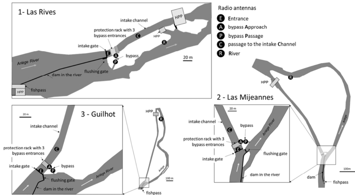
Figure 3: Studied sites and their antenna configurations for downstream passage survey of salmon smolts.
