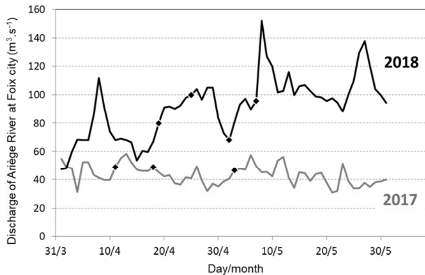
Figure 4: Mean daily discharge of the Ariège River at Foix during the study (dots: days of fish release). The low and median discharge levels (respectively the 5 and 50 percentile flow, Q_{05} and Q_{50} ) for the Ariège River at Foix are respectively 11.8 and 30.3 \text{ m}^3 \cdot \text{s}^{-1} (established from 116 years of data available on http://hydro.eaufrance.fr ).
