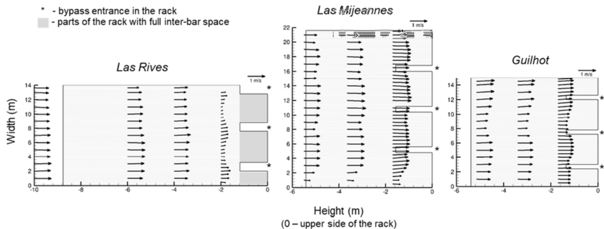
Figure 2: Flow direction and velocity measured with Acoustic Doppler Current Profiler (ADCP) at several transects upstream from the racks (Dewitte et al., 2020; Lemkecher et al., 2018).
