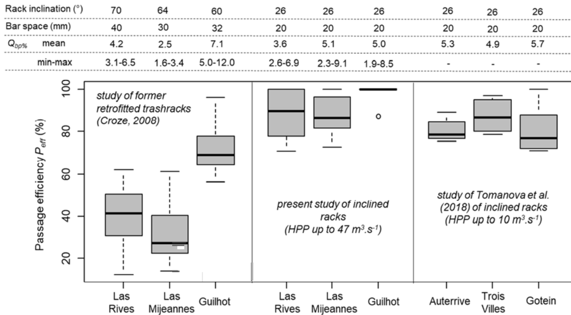
Figure 8: Comparison of the passage efficiency ( P_{eff} ) between the previous and current devices, i.e. retrofitted trashracks (data from Croze, 2008) and horizontally inclined racks on the three studied sites (Wilcoxon tests revealed significant differences with p < 0.001 in all pairwise comparisons), and with three other horizontally inclined racks studied by Tomanova et al. (2018) in smaller HPPs. Both cited studies applied RFID technology (Radio Frequency Identification) and assessed P_{eff} using the number of released fish instead of the number of fish actually passing through the HPP, as we did here, potentially inducing a very minor underestimation of P_{eff} values in both studies.
