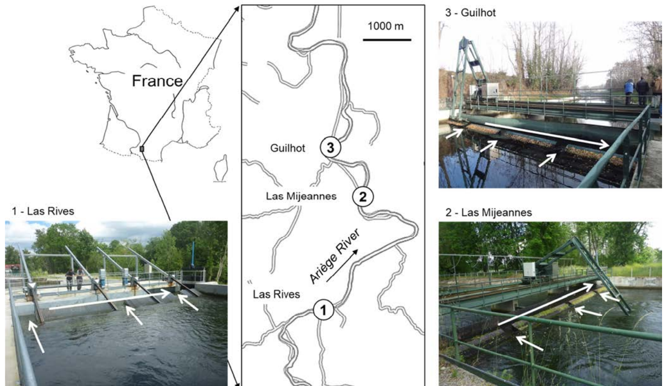
Figure 1: Study area with HPP location and fish protection racks with bypasses (white arrows indicate entrances and bypass, see site coordinates in the text).
