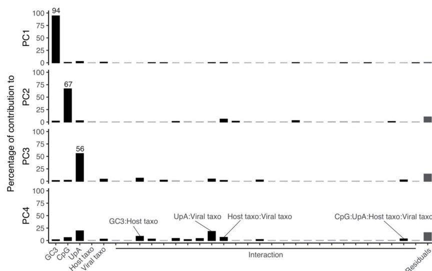
Figure 4. Linear model quantifying the relative contribution of the different variables to the projections of the first four main dimensions of the synonymous codon usage PCA (Figure 1A). Variables included in the linear model are: GC3-content, observed/expected frequency of the CpG dinucleotide, observed/expected frequency of the UpA dinucleotide, host taxonomy at the level of family, viral taxonomy at the level of genus, and all their pairwise interactions. Statistically significant contributions are shown as black bars, stating the percentage of the total explanatory contribution to the correspondent PCA dimension.
