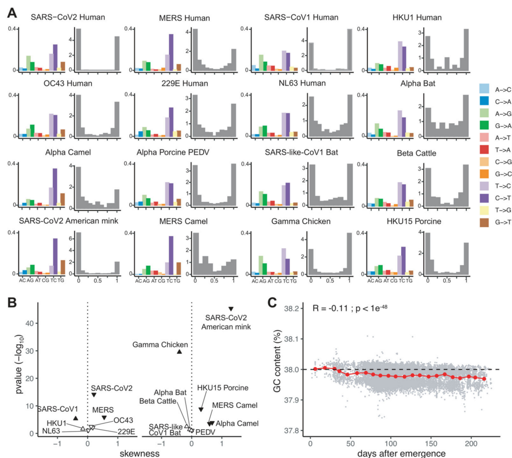
Figure 2. Mutational bias and equilibrium among endemic and recently zoonotic coronaviruses. (A) (left side of each panel) Relative substitution rates for all twelve transition and transversion events, calculated from the total number of SNPs called on the synonymous compartment of a metapopulation composed by all available sequences of the corresponding virus, curated, filtered and aligned. In the x axis, for each of the nucleotide pairs indicated, the frequency of the two substitutions are indicated, e.g.: A→G in light green and G→A in dark green for the AG pair, or T→C in light purple and C→T in dark purple for the TC pair. (right side of each panel) Folded Site Frequency Spectrum (SFS) of G/C-to-A/T substitutions. For each viral metapopulation, the frequencies of SNPs involving a change in GC content called are plotted, the x-axis progressing from GC-enriching to AT-enriching substitutions. (B) Volcano plot of the folded SFS skewness values presented in (A), plotted against the probability that such a value could have been obtained if the corresponding metapopulation were at its mutational equilibrium. The left panel displays CoVs infecting humans while the right panel displays CoVs infecting other mammalian hosts. Downward and upward triangles, respectively, refer to SFS-negative and SFS-positive skewness values. Filled triangles indicate metapopulations with a skewness significantly different from the expected one at mutational equilibrium. (C) Temporal evolution of the SARS-CoV-2 GC-content in the coding genome during the spread of the pandemic. The GC-content of each individual SARS-CoV-2 genome is represented by a gray dot. Red dots represent the average GC-content by time window of 10 days. The results of a Pearson correlation test of GC content over time for the complete data set ( n = 81,963 ) are displayed in the inset.
