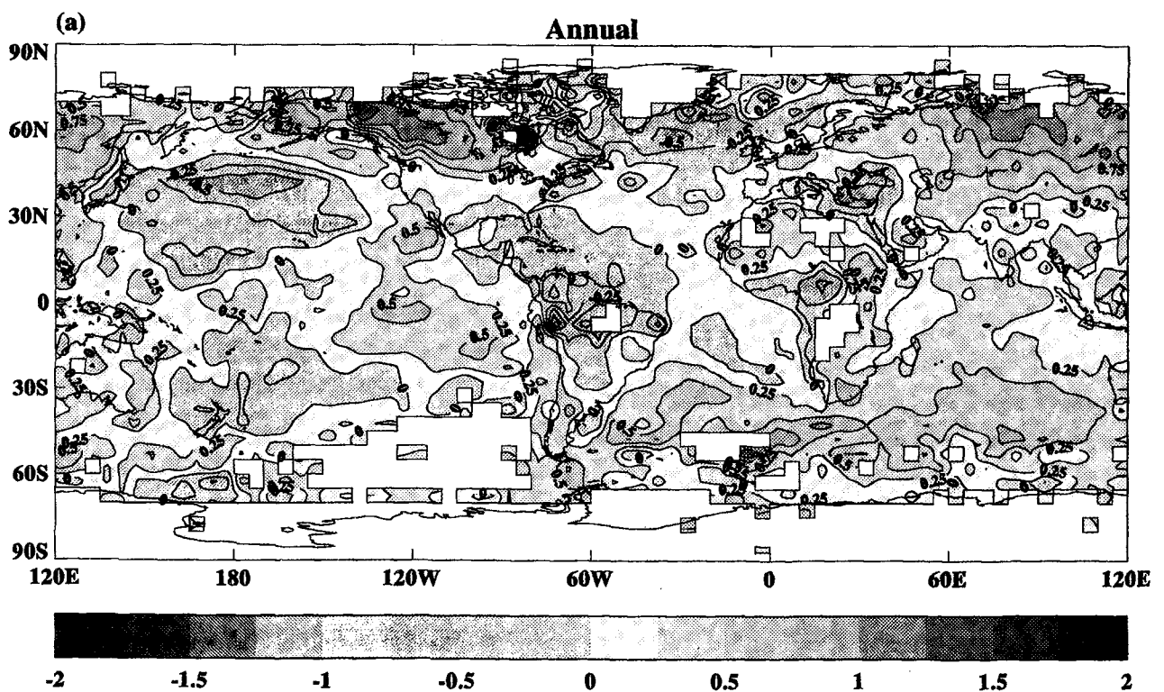
Figure 3.4: Change in surface temperature ( ^{\circ}\text{C} ), from 1955–1974 to 1975–1994: (a) annual; (b) December to February; (c) March to May; (d) June to August; (e) September to November. Sea surface temperatures are from Parker et al. (1995) and land-surface air temperatures are from Jones (1994a).
