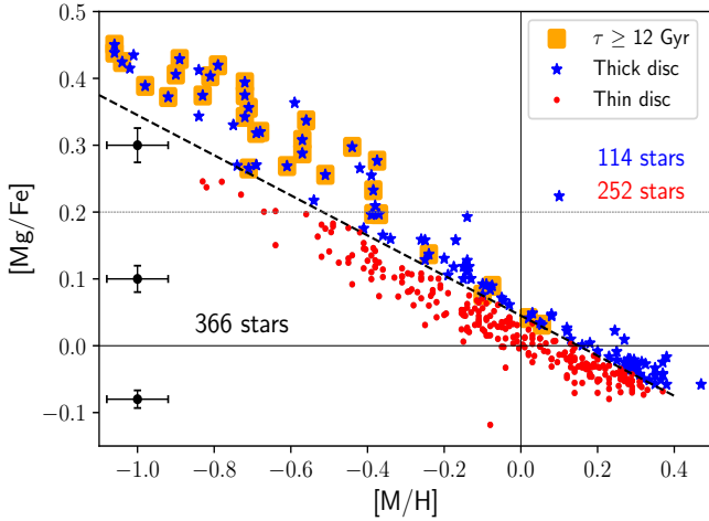
Fig. 3. [\text{Mg}/\text{Fe}] vs. [\text{M}/\text{H}] for our working sample. The stars with ages older than 12 Gyr are highlighted with orange squares. The black dashed line defines the thin (red circles)–thick (blue stars) disc chemical separation. The mean estimated errors are represented on the left-hand side for three different intervals in [\text{Mg}/\text{Fe}] .
