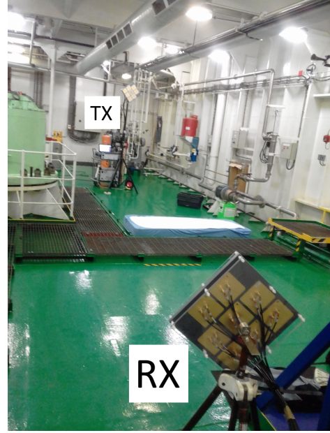
Fig. 12. Measurement setup for fall detection via MIMOSA channel sounder
