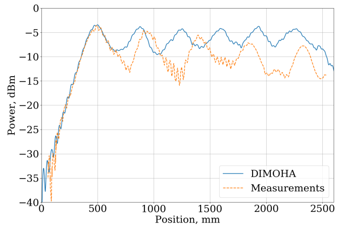
FIG. 5. Time average RF power at F = 220 MHz as function of the longitudinal position inside a 3 m long TWT 33 at time t = 0.7 \mu s. The power is expressed in dBm from watts as P[\text{dBm}] = 10 \log_{10}(P[\text{W}] \cdot 10^3) . Simulations are performed using the measured dispersion relation and interaction impedance of the device.
