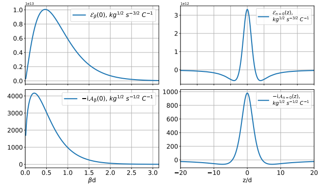
FIG. 4. Amplitude of eigenfields (left column) and shape functions (right column), for the electric field (upper row) and the vector potential (lower row), from Eqs (20)-(23). All panels use the sheath helix dispersion relation and sheath helix interaction impedance from Fig. 2 as function of the phase per pitch \beta d .
