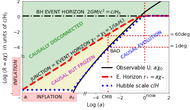
Figure D.7: Extension of Fig.2 to the period of inflation. The FLRW Event Horizon r_* = a\chi_* in Eq.17 (red dashed line) here is also the BHU junction and matches the primordial causal boundary for inflation \chi_* = \chi_\S . Scales larger than r_* are causally disconnected (green shading). Our event horizon today a\chi_* \simeq c/H_\Lambda becomes the BH event horizon (dot-dashed line) in the SW frame.
