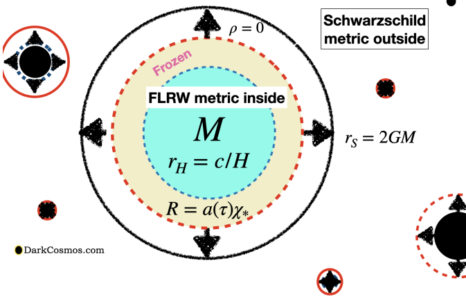
Figure 5: Illustration of the BHU inside the event horizon r_S = 2GM . This is a Schwarzschild (empty) metric outside ( r > R ) and a FLRW metric with a Hubble radius r_H = c/H inside ( r < R ). For a fixed mass the BHU solution in Eq.48 requires R = [r_H^2 r_S]^{1/3} . There is a region with matter outside the Hubble radius R > r > r_H (yellow shading). This solves the horizon problem in Cosmology and is a source for perturbations that enter the horizon as the metric expands, creating LSS and BAO in Cosmic Maps, pretty much like what is usually assumed for Cosmic Inflation.
