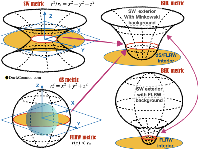
Figure 4: Spatial representation of ds^2 = (1 + 2\Phi)^{-1} dr^2 + r^2 d\theta^2 2D metric embedded in 3D flat space for: deSitter (dS, bottom left, 2\Phi = -r^2/r_*^2 ), FLRW ( r(\tau) < r_* , blue sphere inside dS), Schwarzschild (SW, top left, 2\Phi = -r_*/r ) and two versions of the combined BHU metrics. Yellow region shows the projection coverage in the (x, y) plane. In the top right figure we show a BHU with dS (or FLRW) interior and SW metric exterior joint at the Event Horizon r_* = 2GM = 1/H_\Lambda (red circles). The BHU solution has in general two nested FLRW metrics join by SW metric (bottom right). See Appendix A for a more detailed explanation.
