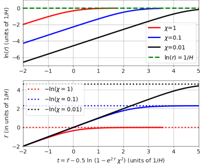
Figure 3: Logarithm of physical radius r = a(\tau)\chi (top) and comoving time \tau (bottom) as a function of SW time t in Eq.34 for a(\tau) = e^{\tau H_\Lambda} and different values of \chi . All quantities are in units of 1/H_\Lambda . For early time or small \chi : \tau \simeq t . A fix \chi acts like an Horizon: as t \Rightarrow \infty we have \tau \Rightarrow -\ln \chi (dotted), which freezes inflation to: r = a\chi \Rightarrow e^{-\ln(H_\Lambda \chi)} \chi = 1/H_\Lambda (dashed).
