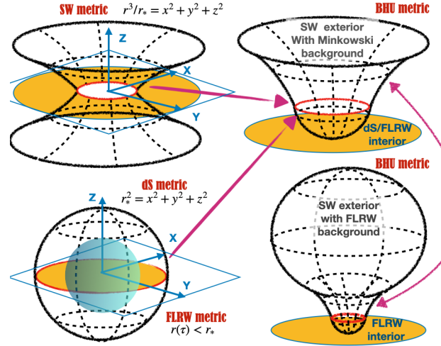
Figure 5. Spatial representation of ds^2 = (1+2\Phi)^{-1} dr^2 + r^2 d\theta^2 2D metric embedded in 3D flat space for: deSitter (dS, bottom left, 2\Phi = -r^2/r_*^2 ), FLRW ( r(\tau) < r_* , blue sphere inside dS), Schwarzschild (SW, top left, 2\Phi = -r_*/r ) and two versions of the combined BHU metrics. Yellow region shows the projection coverage in the (x, y) plane. In the top right figure we show a BHU with dS (or FLRW) interior and SW metric exterior joint at the Event Horizon r_* = 2GM = 1/H_\Lambda (red circles). The BHU solution has in general two nested FLRW metrics joined by SW metric (bottom right). See Appendix A.
